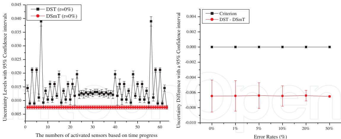
(a) Uncertainty levels of two cases with r=0\% (b) Comparison Uncertainty levels of two cases
