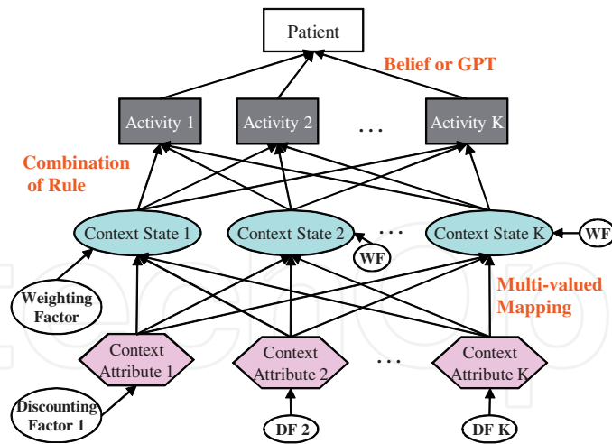
Fig. 3. An Evidential Fusion Network (EFN)
