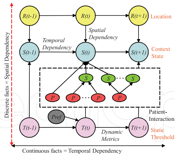
Fig. 1. A Relation-dependency approach
