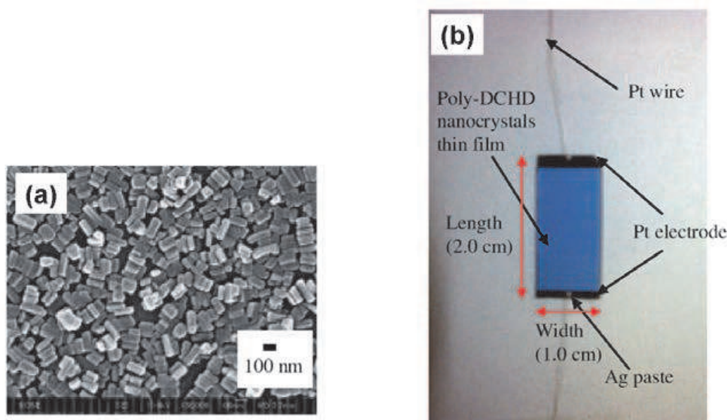
Fig. 6. (a) Single layered poly(DCHD) nanocrystals on quartz slide glass. (b) Image of the specimen for conductivity measurement of single layered poly(DCHD) nanocrystals.
