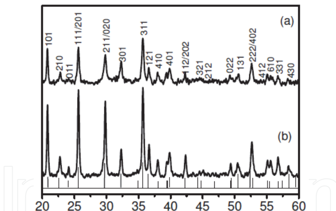
Fig. 2. XRD patterns of the \text{LiFePO}_4 , (a) nano-rods obtained by 8 min reaction; and (b) hierarchical nanostructure obtained by 20 min reaction time at 400 °C.
