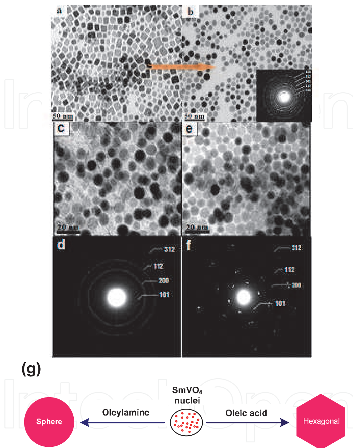
Fig. 8. Effects of the reaction temperature and surfactants with different functional groups on the shape control. TEM images of 15 nm-sized SmVO 4 nanocrystals synthesized at different temperatures for 16 h: (a) nanocubes at 150 °C and (b) nanospheres at 180 °C;(Nguyen et al. 2009a) TEM images and SAED patterns of the SmVO 4 nanocrystals synthesized from a 1:1 mixture of Sm(OA) 3 and VO 4 (TOA) 3 in toluene using various surfactants: (c,d) oleylamine, 17 nm nanospheres, (e,f) oleic acid, 17 nm nanohexagons, and (g) Schematic illustration for the shape control of the SmVO 4 nanocrystals (Nguyen et al. 2009b).
