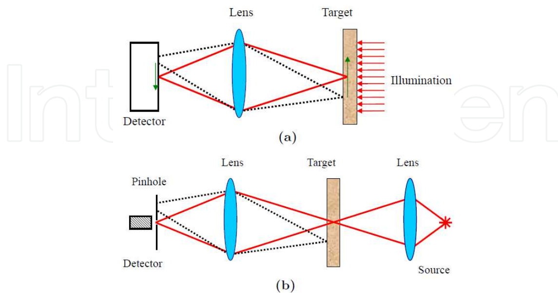
Fig. 1. Different types of microscopy: (a) wide-field microscopy; (b) confocal microscopy. (Xi, Rajwa et al. 2007)
