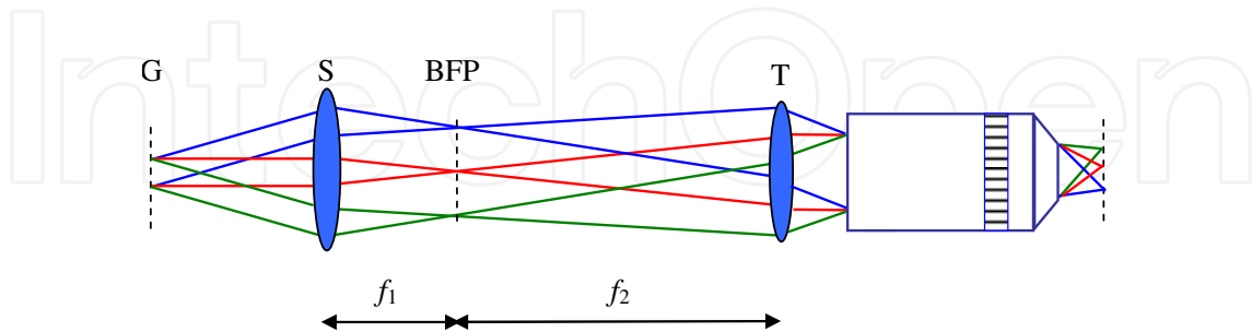
Fig. 3. The configuration of a confocal laser scanning microscopy system. G: Galvanometer; S: scan lens; BFP: back focal plane; T: tube lens; f_1 : focal length of S; f_2 : focal length of T.
