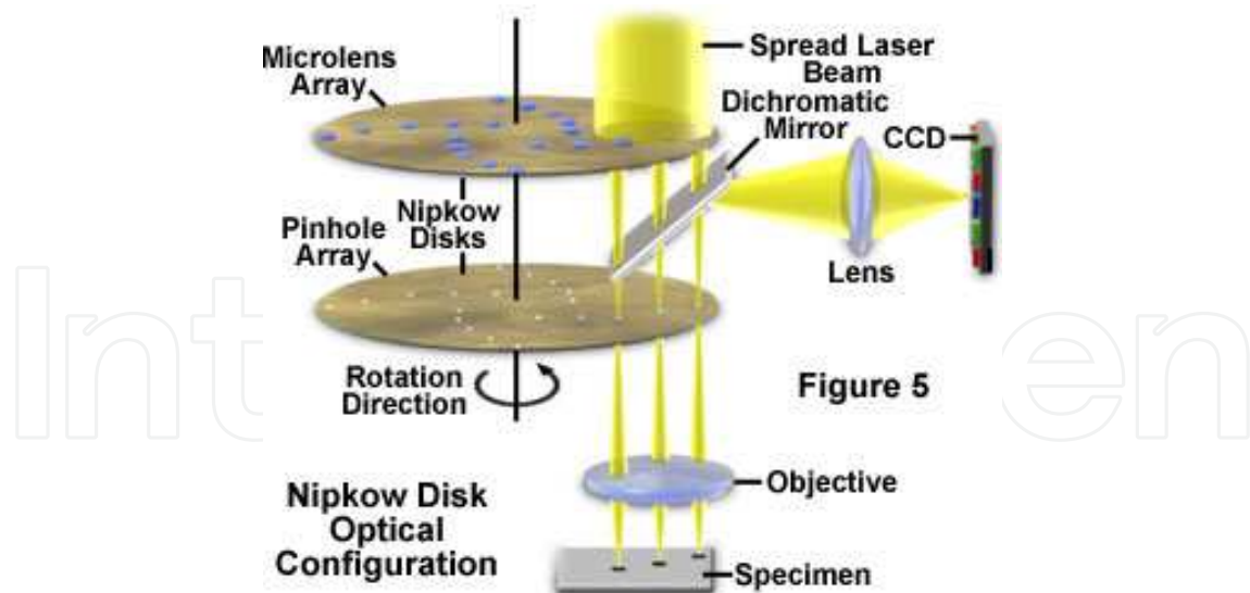
Fig. 19. Schematic diagram of the Nipkow disk scanning system ( http://www.microscopyu.com/articles/confocal/confocalintrobasics.html ).
