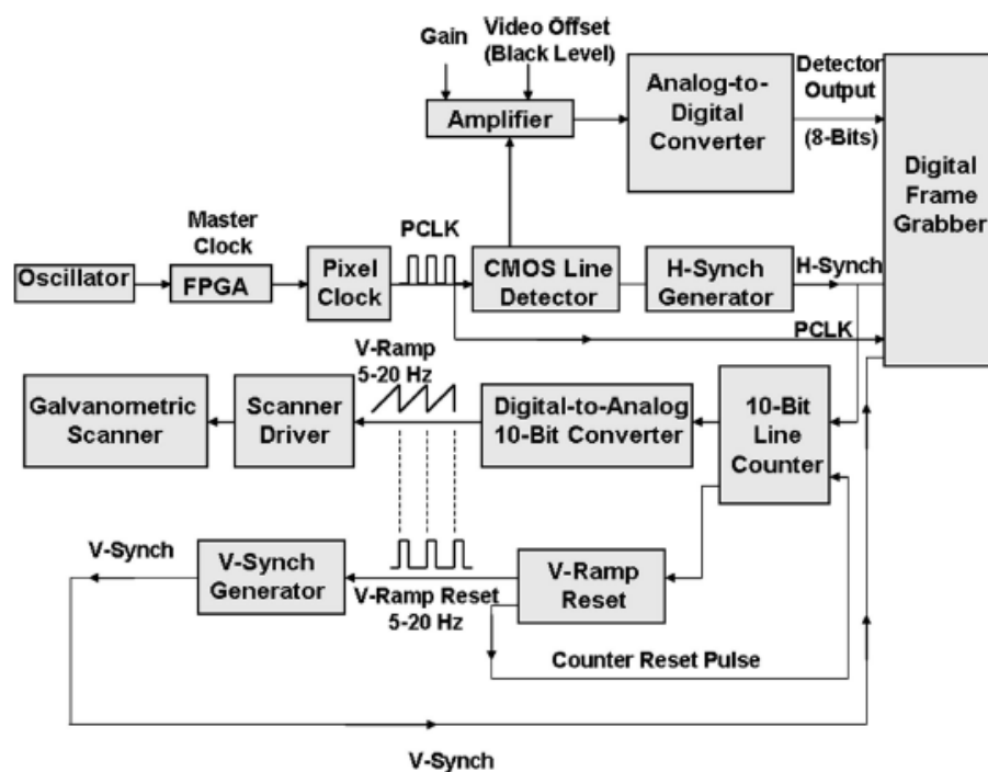
Fig. 18. Schematic diagram (a) and control circuit (b) of the theta-line scanning system. A 1024-element CMOS line camera was used for data collection (Dwyer, DiMarzio et al. 2007) Image courtesy of OSA.
