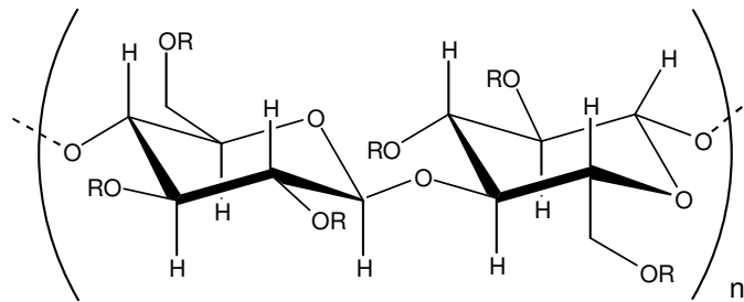
Fig. 1. Chemical structure of CA.
