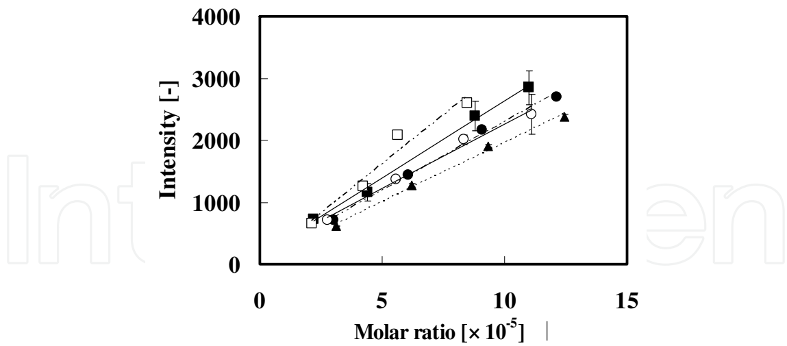
Fig. 15. Relationships between molar ratio and fluorescent intensity of perylene mixed with additives: GTA (■), TEGDA (●), BGDA (○), paraffin liquid (□) and PEG (▲).
