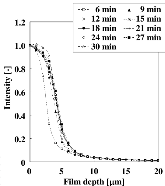
Fig. 25. Relationship between the depth of CCA sample and I_s at several times after addition of perylene/GTA mixture.
