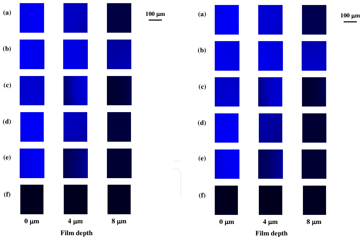
Fig. 16. Chemical images of CCA sample at several depths 9 minutes after addition of perylene/additive mixtures: (a) /GTA, (b) /TEGDA, (c) /BGDA, (d) /paraffin liquid, (e) /PEG and (f) control (without addition).
