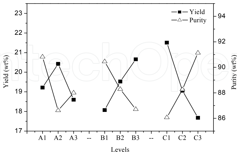
Fig. 1. Effect of factors on the yield and purity of recovered phytosterols under different levels.
