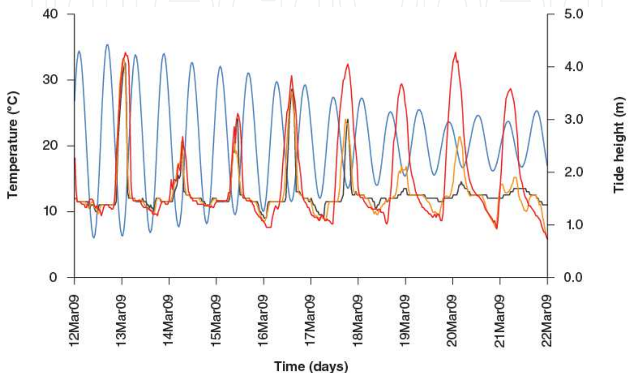
Fig. 6. Example of robolimpet data from an exposed rocky shore in Biarritz (SW France) taken between March 12 th 2009 and March 22 nd 2009. Times are in GMT. The black, orange and red lines show temperatures as measured by low-, mid- and high-intertidal loggers. Tidal heights are shown by the blue line.
