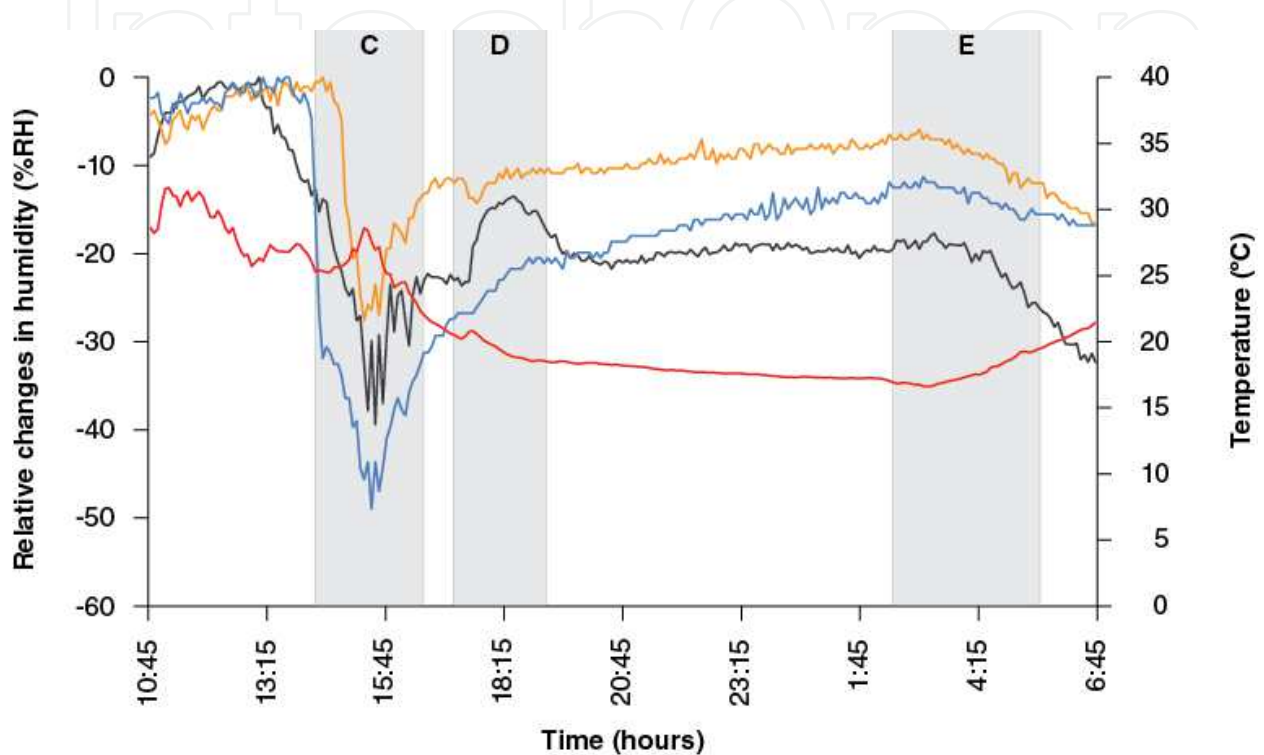
Fig. 9. Comparison between water loss measured in a live limpet ( Patella vulgata - black line) and water loss as recorded by two biomimetic desiccation loggers (blue and orange lines) on a supralittoral rocky surface at Lavra (NW Portugal) on June 23 rd -24 th 2010. The temperature trajectory of the limpet is shown in red. Period C corresponds to strong afternoon sun, which was followed by sunset at D. Temperatures decreased gradually during the night, but rose at sunrise (E), causing evaporative water loss in the live animal and in the biomimetic loggers.
