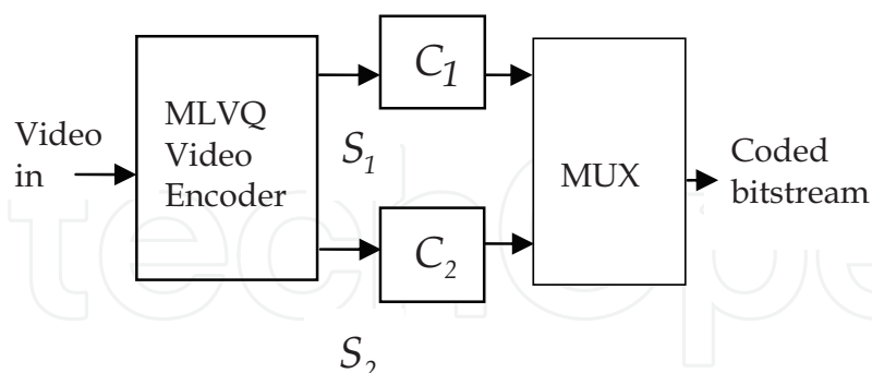
Fig. 10. UEP scheme for MLVQ video codec
