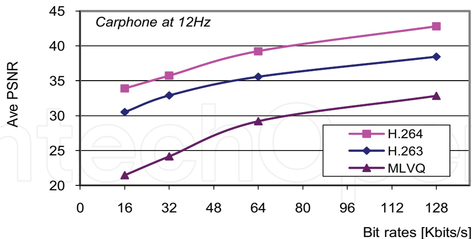
Fig. 13. "Carphone" over noiseless channel
