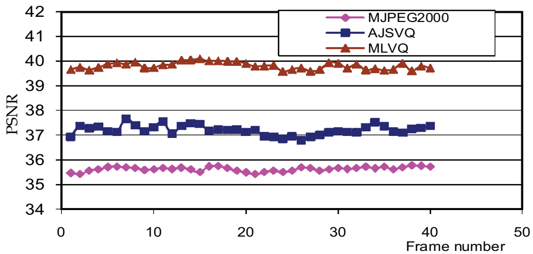
Fig. 11. Relative performance of "Miss America" at 8 fps
