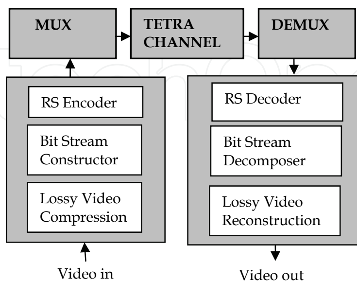
Fig. 9. Block diagram of MLVQ video transmission
