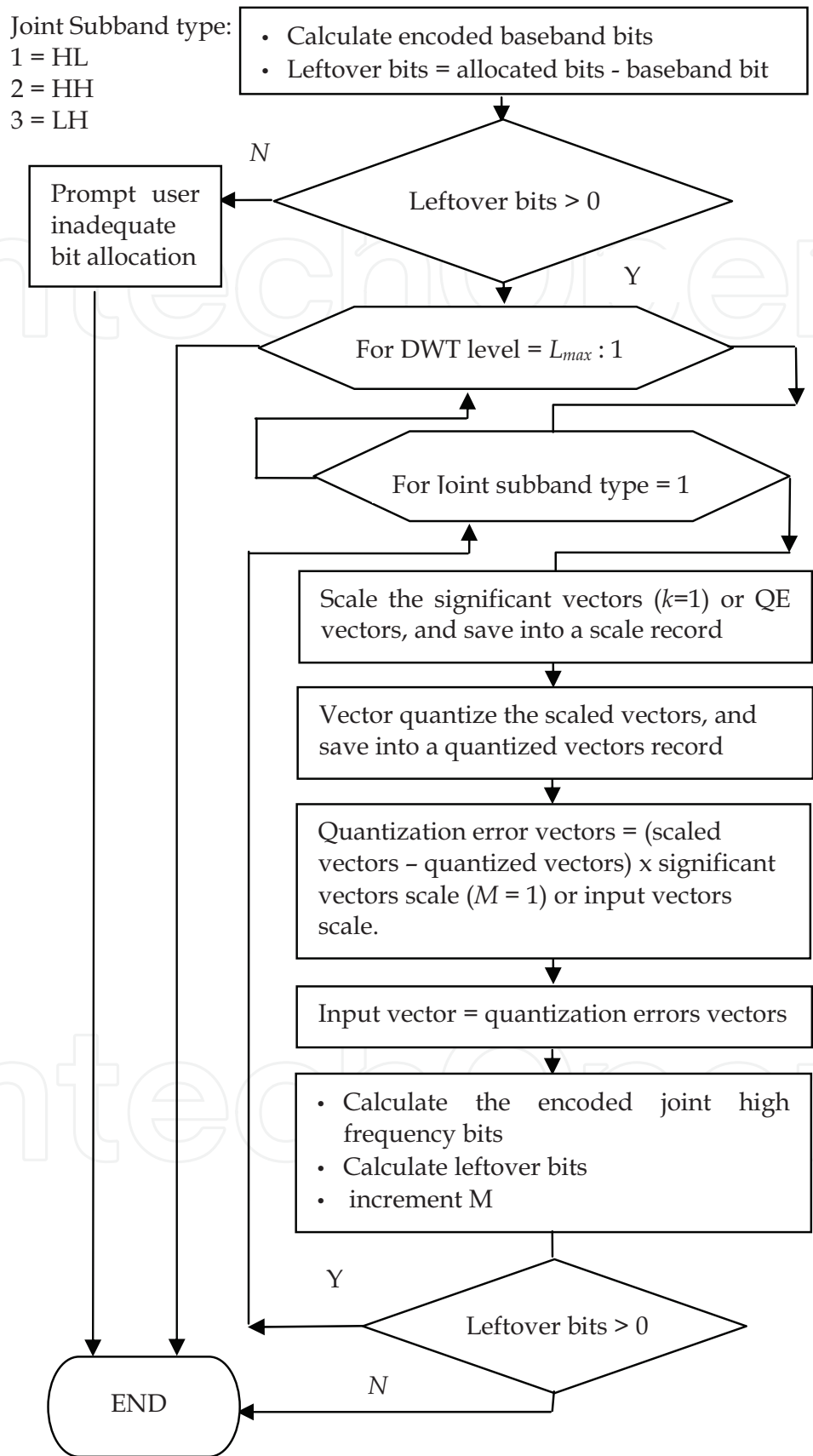
Fig. 8. Flow diagram of MLVQ algorithm
