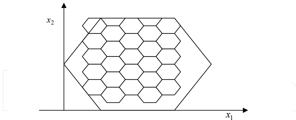
Fig. 1. Two-dimensional hexagonal lattice
