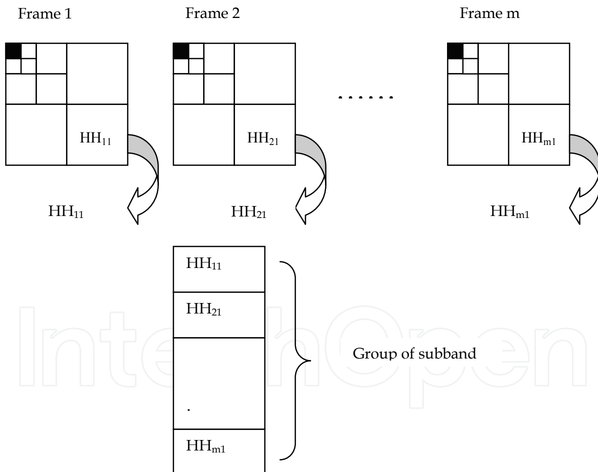
Fig. 6. Joining subband significant coefficients in a GOP
