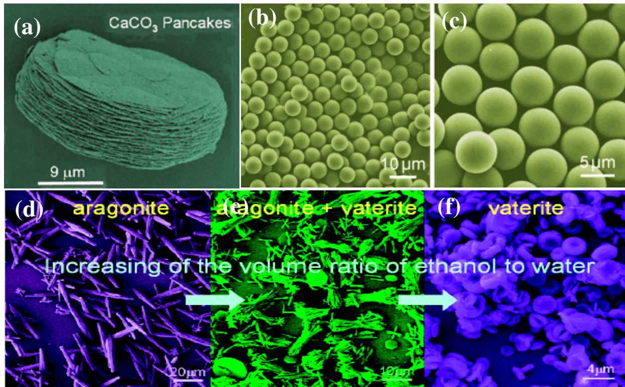
Fig. 29. SEM images of the \text{CaCO}_3 : (a) calcite pancakes; (b,c) monodisperse \text{CaCO}_3 (vaterite) microspheres; (d-f) vaterite superstructures and aragonite rods. Reproduced with permission from Adv. Mater. 2005 , 17 , 1461, Angew. Chem. Int. Ed. 2006 , 45 , 3977, and Chem. Mater. 2006 , 18 , 115. Copyright 2010 ACS and VCH.
