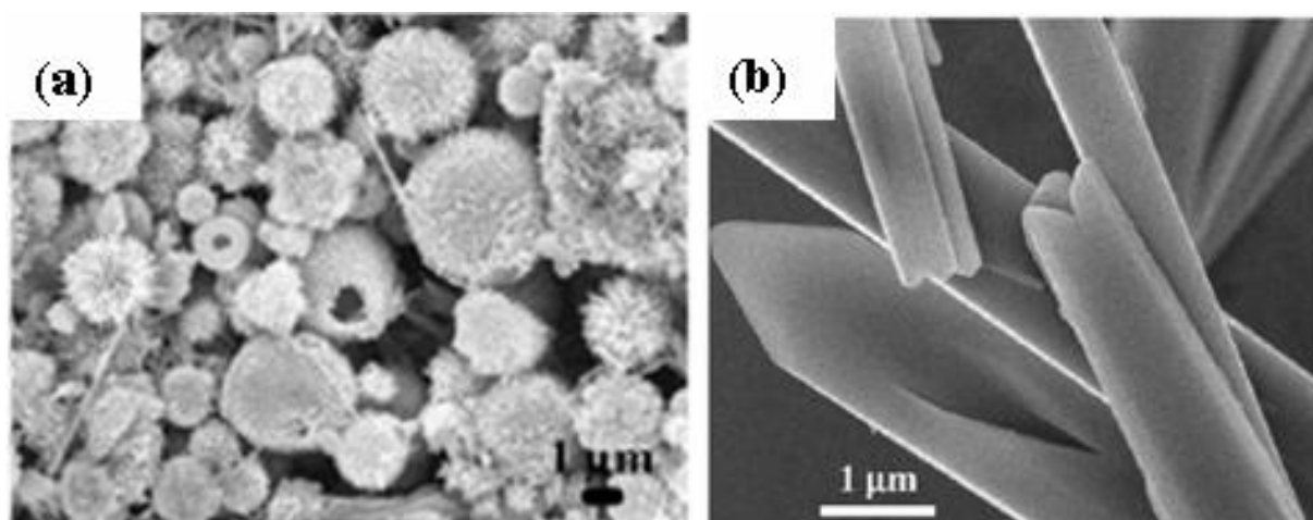
Fig. 1. (a) SEM micrograph of the hierarchically nanostructured HA hollow spheres, (Reproduced with permission from Eur. J. Inorg. Chem. 2009 , 5522. Copyright 2009 VCH.) and (b) TEM micrograph of the HA microtubes. (Reproduced with permission from Mater. Lett. 2008 , 62, 1642. Copyright 2008 Elsevier)
