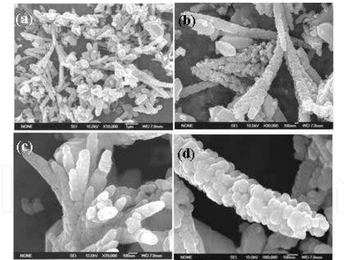
Fig. 13. SEM micrographs of \text{SrCO}_3 prepared by microwave heating an aqueous solution of (\text{NH}_4)_2\text{CO}_3 , \text{Sr}(\text{NO}_3)_2 and EDA at 90^\circ\text{C} for 20 min. (a) at a lower magnification, (b) at a higher magnification, (c) the top view of the branch-like morphology, (d) a typical single branch assembled from nanoparticles. Reproduced with permission from Mater. Lett. 2008 , 62, 2512. Copyright 2008 Elsevier.
