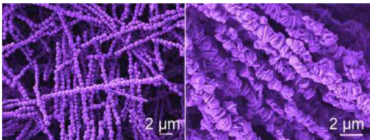
Fig. 28. SEM images of the one-dimensional assembly of Ni_xCo_{1-x} alloy microparticles. Reproduced with permission from Nano Research 2008 , 1 , 303. Copyright 2008 springer .
