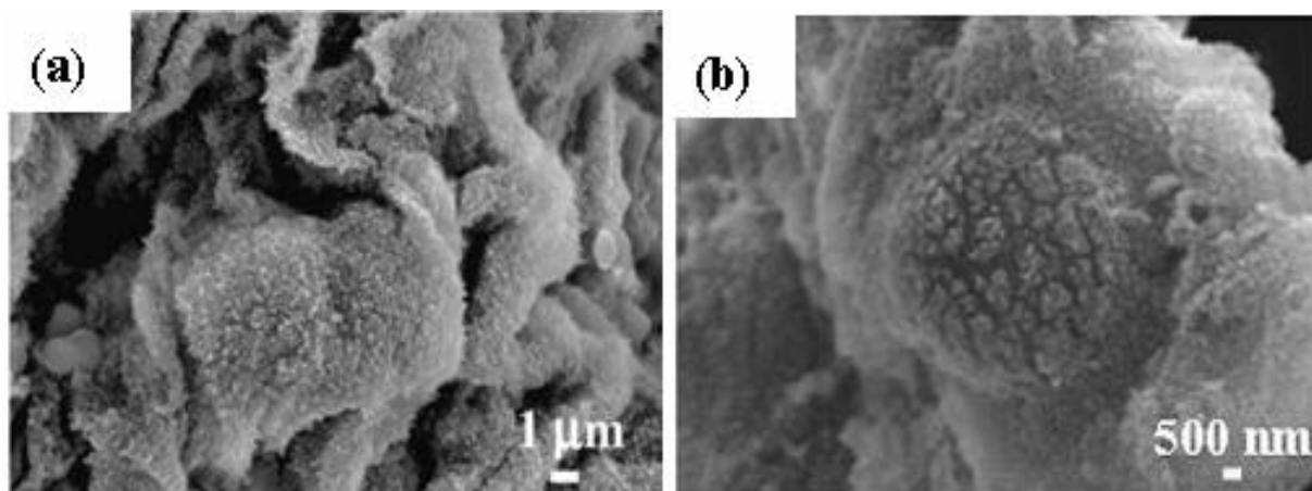
Fig. 4. SEM micrographs of (a) the cellulose-calcium silicate nanocomposites and (b) the cellulose-HA nanocomposites. Reproduced with permission from Carbohydr. Polym. 2010 , 80 , 270 and Carbohydr. Res., 2010 , 345 , 1046. Copyright 2010 Elsevier .
