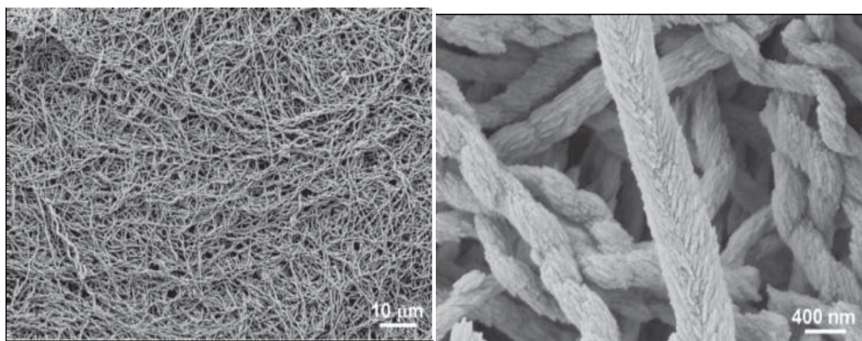
Fig. 25. Helical nanoparticle superstructures. a , The helical nanofibers formed at room temperature with PEG-b-DHPOBAEE, 1 \text{ gL}^{-1} , starting \text{pH}=4 , [\text{BaCl}_2] = 10 \text{ mM} . b , Detailed surface structure. Reproduced with permission from Nature Materials 2005 , 5 , 51. Copyright 2005 Nature Publishing Group.
