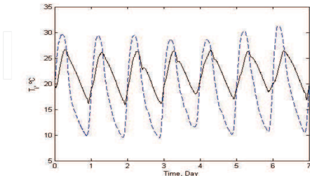
Fig. 8. Measured (solid line) and simulated (dotted line) air temperature by means of a gray box model
