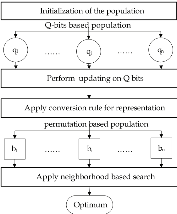
Fig. 2. The algorithm framework for permutation-based scheduling problems
