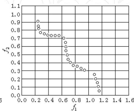
Fig. 7. Pareto front on TNK using LEA
