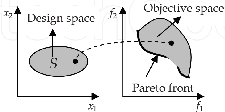
Fig. 2. Mapping from design space to objective space.
