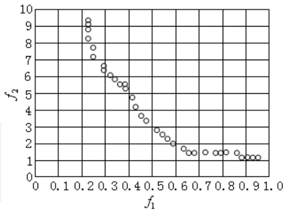
Fig. 8. Pareto front on CE using NSGA-II
