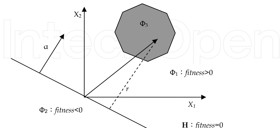
Fig. 3. Transformation of searching space.
