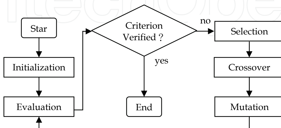
Fig. 1. Evolutionary algorithm flow chart
