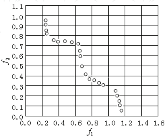
Fig. 6. Pareto front on TNK using NSGA-II
