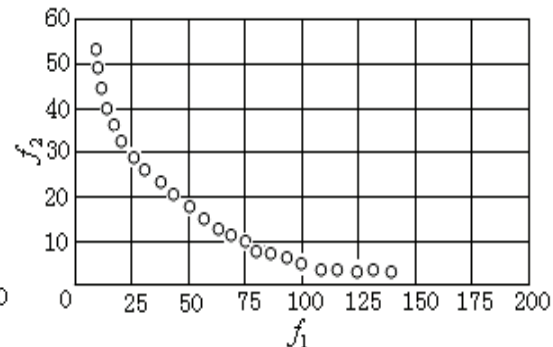
Fig. 5. Pareto front on BNH using LEA
