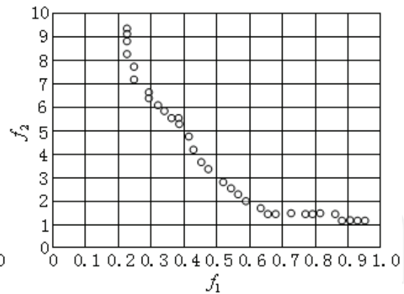
Fig. 9. Pareto front on CE using LEA
