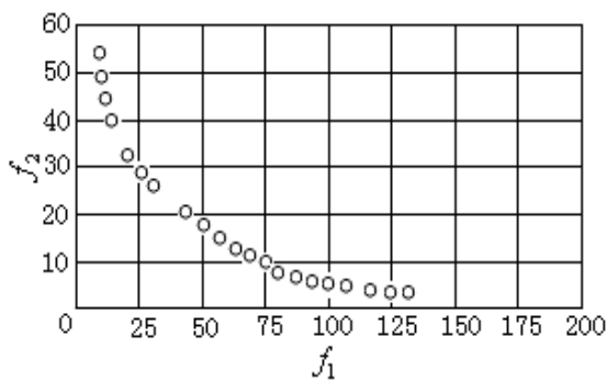
Fig. 4. Pareto front on BNH using NSGA-II
