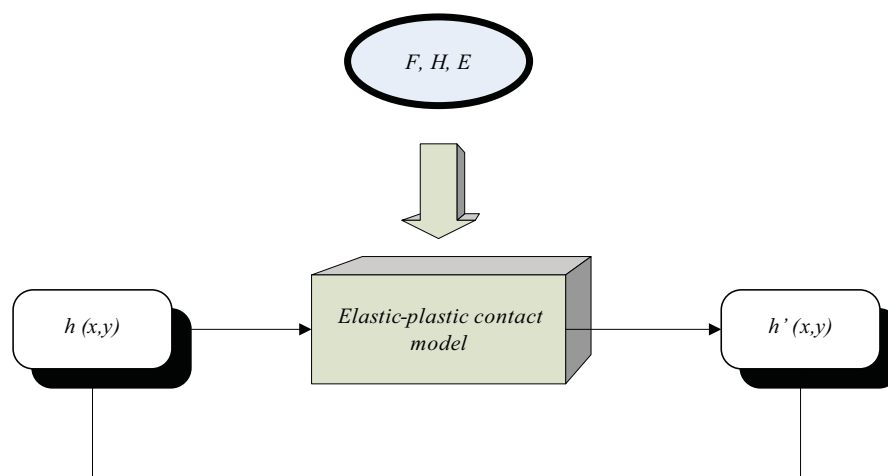
Fig. 5. The model of the surface topography changes due to running-in of a rolling contact proposed by Jamari (2006)
