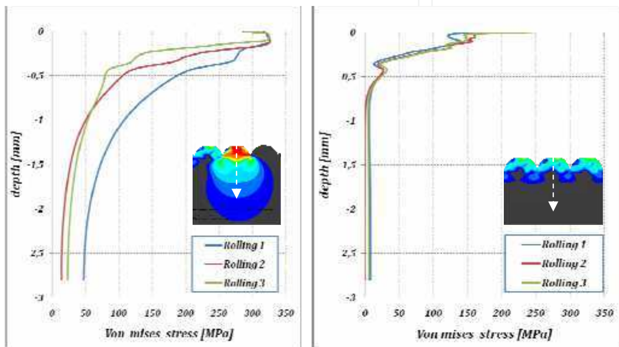
Fig. 9. von Mises Stress analysis (a) during rolling contact and (b) residual stress after the rolling contact finish.
