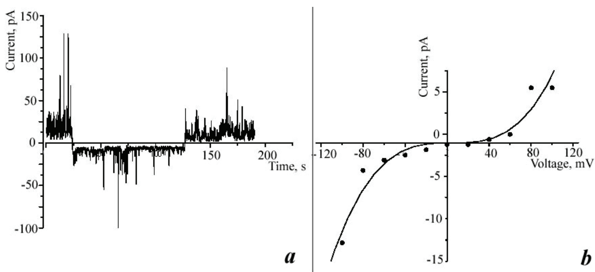
Fig. 2. Current fluctuations ( a ) and current-voltage characteristics ( b ) of a lipid bilayer from phosphatidylcholine (20 mg/ml) in presence 2 ng/ml recombinant LIF(pro). External solution: 1M KCl, 10 mM CaCl 2 ; 40 mM Tris-Hepes, pH 7.2; voltage 100 and -100 mV.
