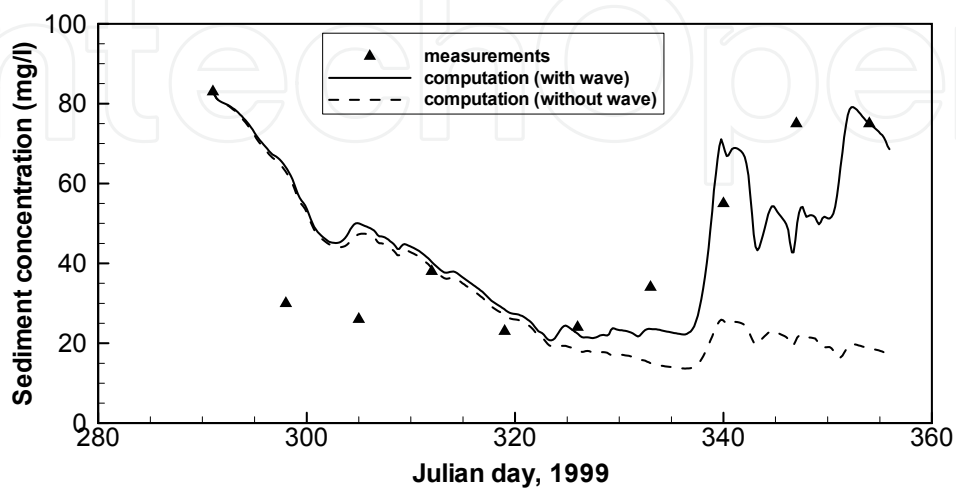
Fig. 12. Suspended sediment concentration at Station DH1
