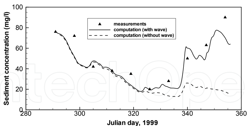
Fig. 13. Suspended sediment concentration at Station DH2
