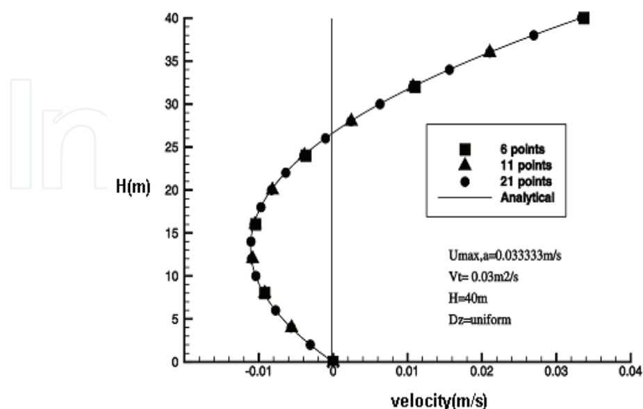
Fig. 2. Comparison of the analytical solution and the numerical simulation of wind-driven flow
