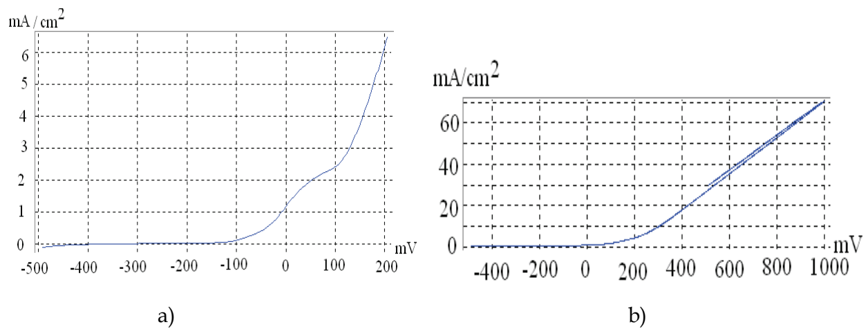
Fig. 5. Polarization curves: a) Ni in NaCl 3% solution, b) Ni/ZrO 2 in NaCl 3% solution
