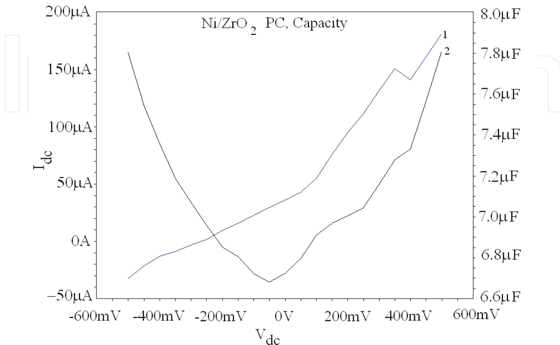
Fig. 15. Polarization curve (1) and variation of capacity (2) of nanocomposite thin films
