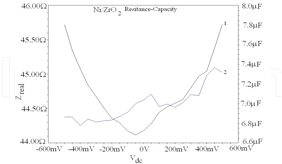
Fig. 13. Variation of capacity (1) and resistance (2) of nanocomposite thin films versus applied potential
