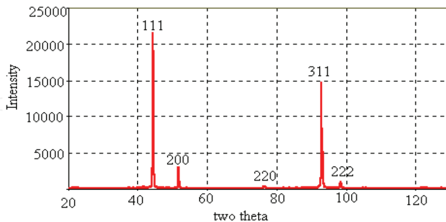
Fig. 4. X-ray diffraction pattern of electrodeposited nickel film with 10 % alumina nanoparticles
