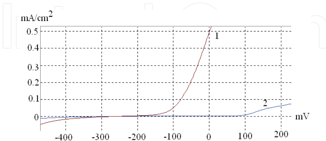
Fig. 8. Polarization curves - Overlapping: Ni/ZrO 2 in Na 2 SO 4 0.1 M solution (1), Ni/ZrO 2 in NaCl 3% solution (2)
