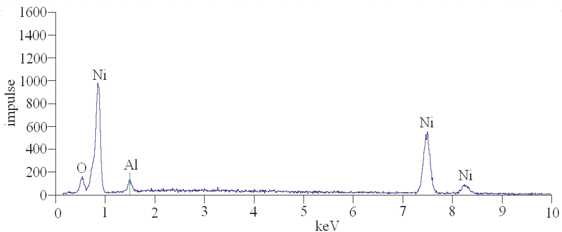
Fig. 3. EDAX spectrum of electrodeposited film with alumina nanoparticles
