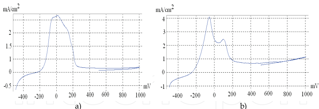
Fig. 7. Polarization curve Ni in H 2 SO 4 0.1 N solution, b) Ni/ZrO 2 in H 2 SO 4 0.1 N solution
