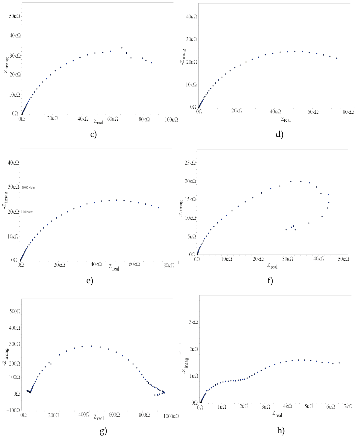
Fig. 12. Representation of Impedance Spectroscopy (Nyquist diagram) for the experimental system of Ni/ZrO 2 in Na 2 SO 4 0.1 M solution at t = 0 s (a), 1h(b), 2 hrs(c), 3hrs(d), 4 hrs(e), 24hrs (f), 46 hrs(g), 47hrs(h)
