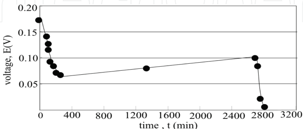
Fig. 10. Voltage variation on time
