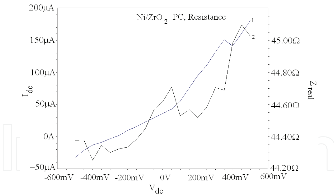
Fig. 14. Polarization curve (1) and variation of resistance (2) of nanocomposite thin films
