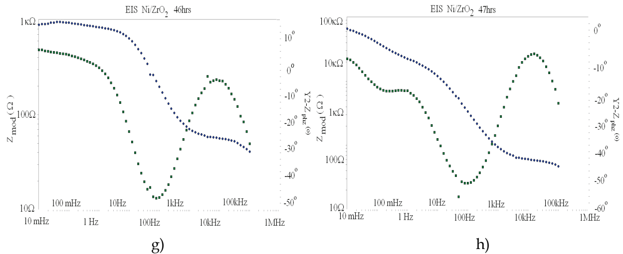
Fig. 11. Representation of Impedance Spectroscopy (BODE Diagram) for the experimental system of Ni/ZrO 2 in Na 2 SO 4 0.1 M solution at t = 0 s(a), 1h(b), 2 hrs(c),3h(d), 4 hrs(e), 24h(f), 46 hrs(g), 47(h)
