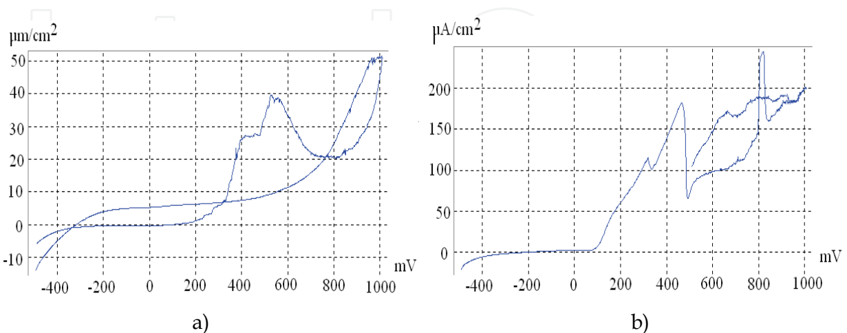
Fig. 6. Polarization curve: a) Ni in Na 2 SO 4 0.1 M solution, b) Ni/ZrO 2 in Na 2 SO 4 0.1 M solution
