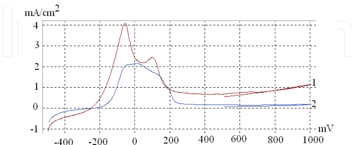
Fig. 9. Polarization curves: Ni/ZrO 2 in H 2 SO 4 0.1 N solution (1), Ni in H 2 SO 4 0.1 N solution (2) - Overlapping
