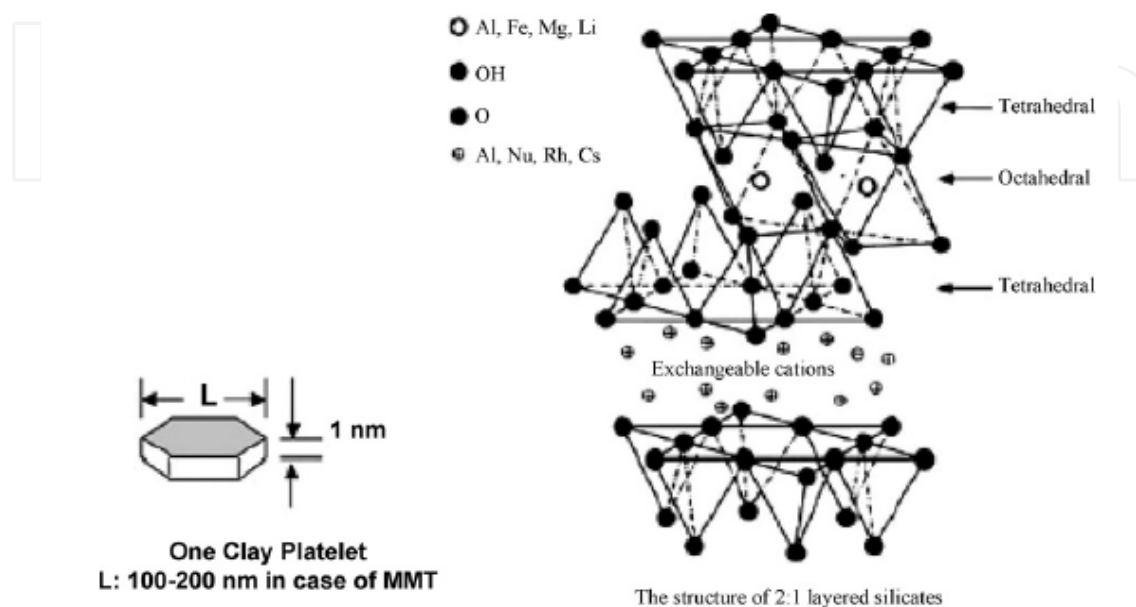
Fig. 1. Structure of 2:1 layered silicate showing two tetrahedral sheets of silicon oxide fused to an octahedral sheet of aluminum hydroxide.
