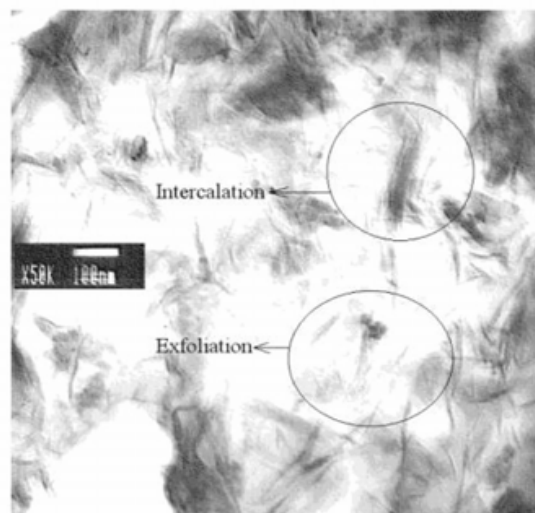
Fig. 9. Transmission electron microscopy of CLMA5.
