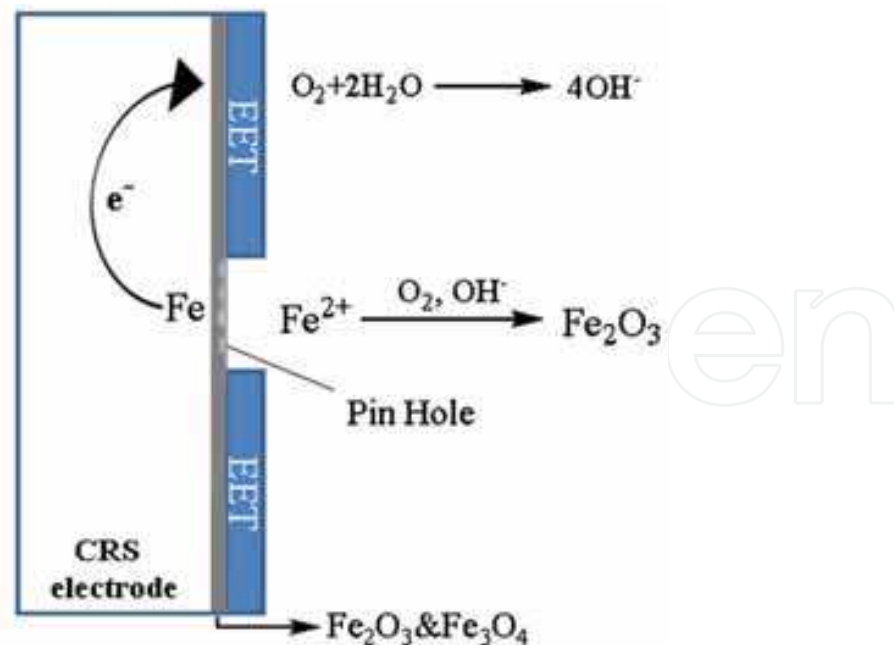
Fig. 20. Schematic diagram of mechanism of the CRS passivation by EET coatings.
