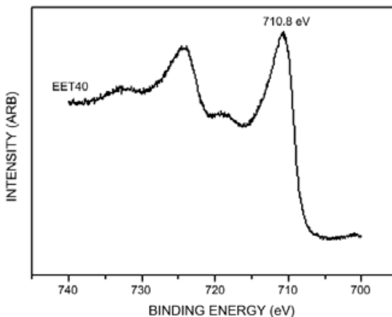
Fig. 19. ESCA Fe 2p core spectrum of EET40.
