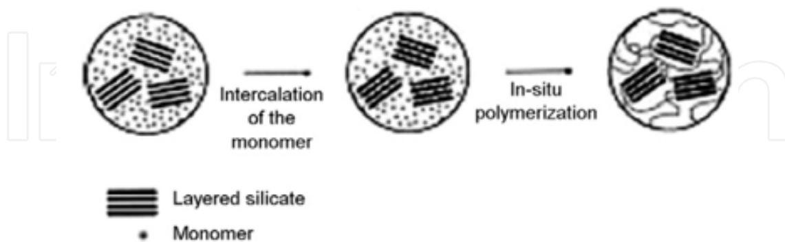
Fig. 6. Schematic representation of a PLS nanocomposite obtained by in-situ polymerization.
