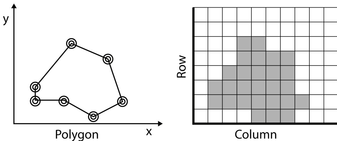
Fig. 1. Tesselation of a polygon to create a raster data type
