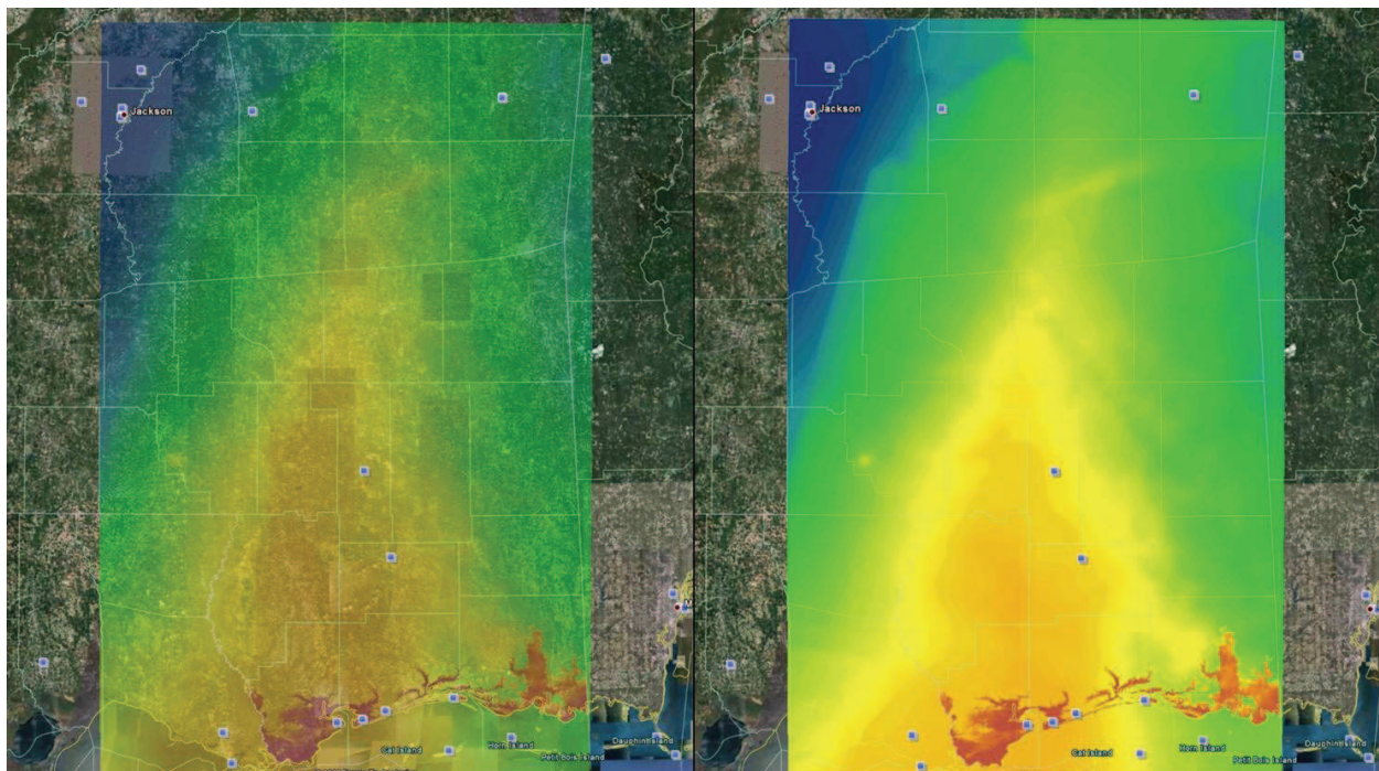
Fig. 2. DESM model output as a KML output file overlaid on Google Earth™
