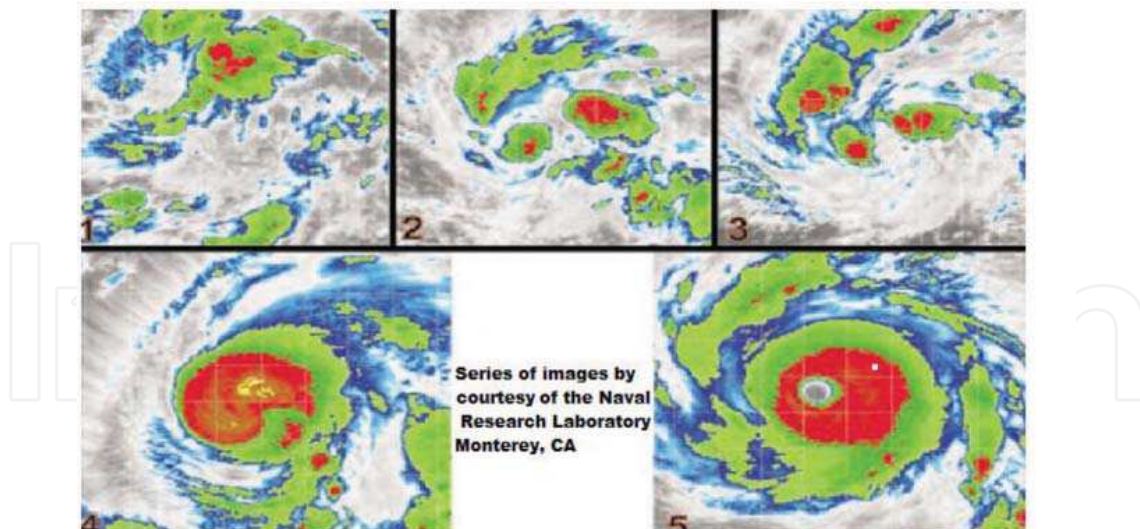
Fig. 4. Series of images of Hurricane Floyd, 1999 (Naval Research Laboratory )
