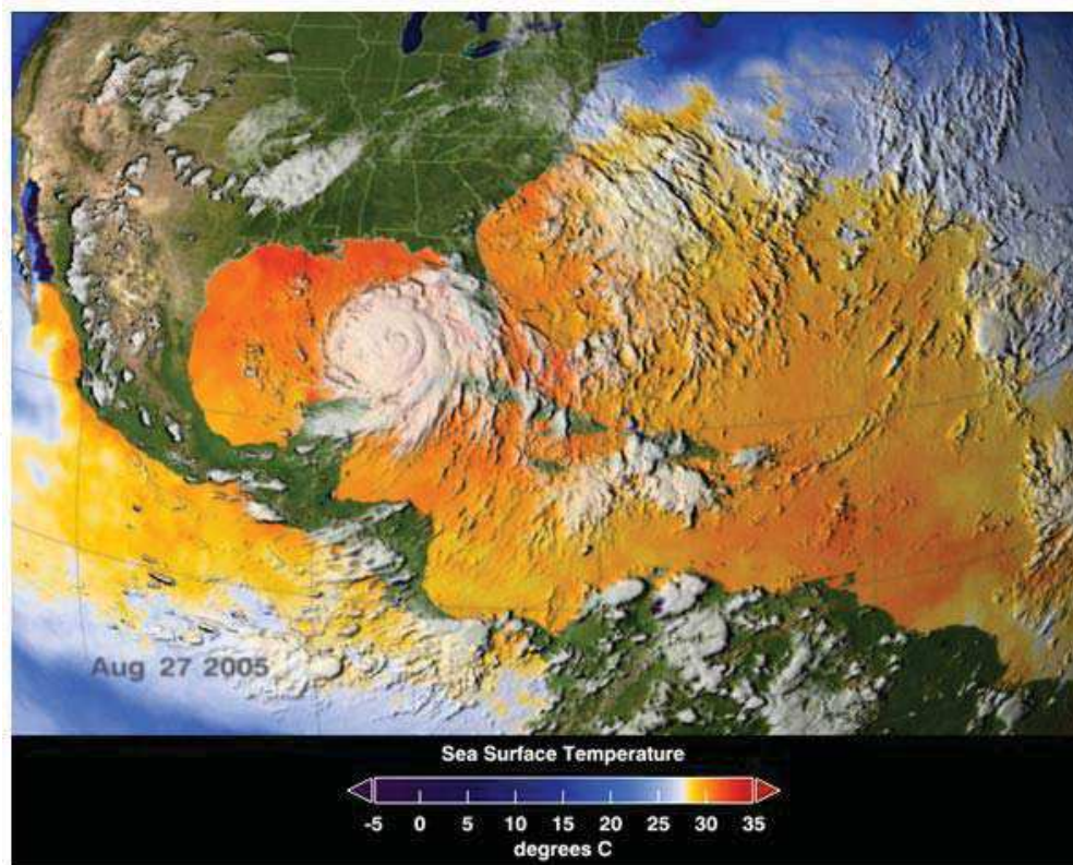
Fig. 2. Hurricane Katrina and the Sea Superficial Temperature
