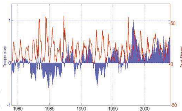
Fig. 7. Superficial Sea Temperature vs Dust Storms (1979 – 2004)
