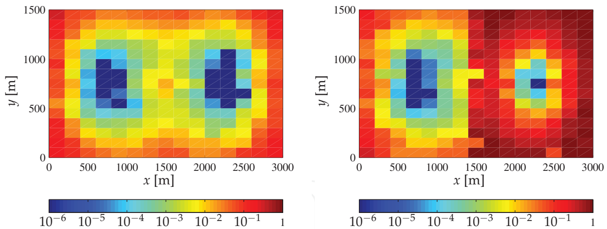
Fig. 7. Outage probability map for a) \gamma = [1, 1] bits/s/Hz and b) \gamma = [1, 1] bpcu
