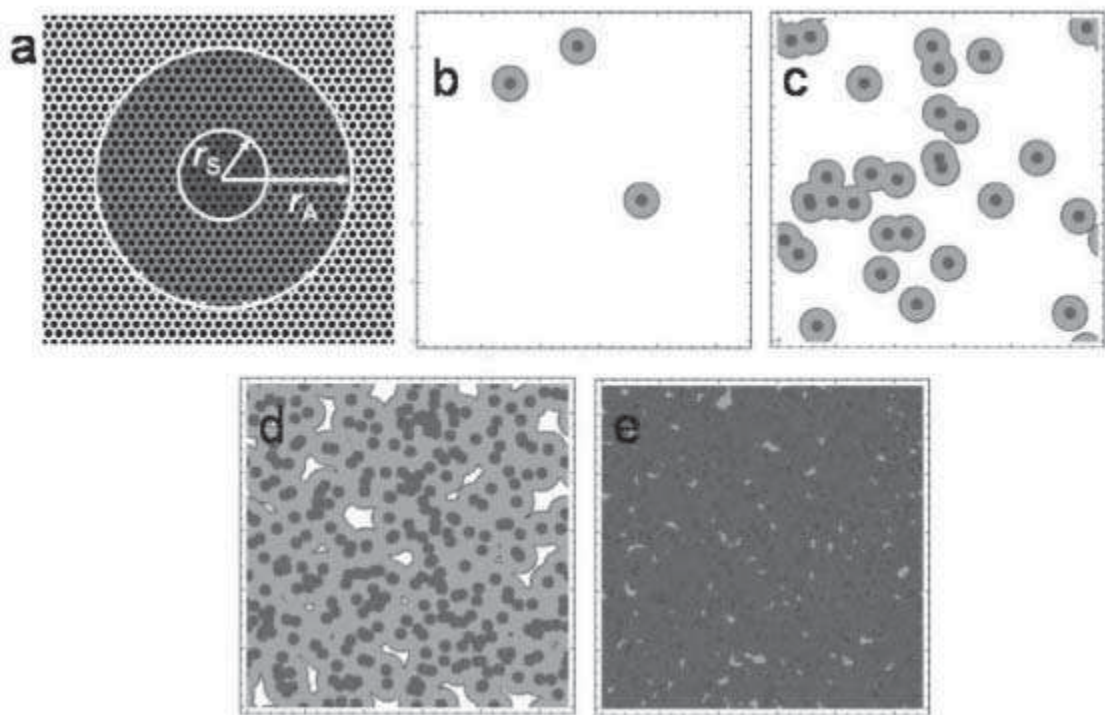
Fig. 8. (a) The two length scales ( r_A and r_S ) describing the evolution of the D band intensity with disorder induced by the impact of Ar^+ ions in graphene. Panels (b) to (e) correspond to the same ion doses in panels (b) to (e) in Figure 3. (Luchese et al. (2010))
