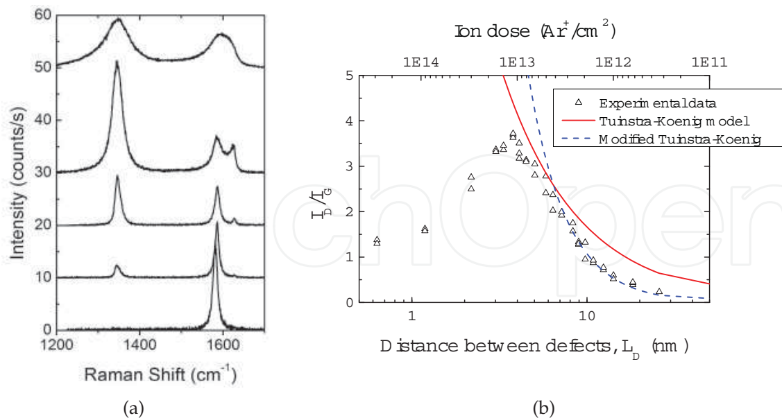
Fig. 4. (a) Raman spectra of a monolayer graphene bombarded with low energy (90 eV) argon ions measured with a 514 nm laser. From bottom to top, curves correspond to zero, 10^{11} , 10^{12} , 10^{13} and 10^{14} \text{Ar}^+/\text{cm}^2 dose. (b) Comparison between experimental I_D/I_G data and both original and modified Tuinstra-Koenig relations for disorder in carbon structures (see text).
