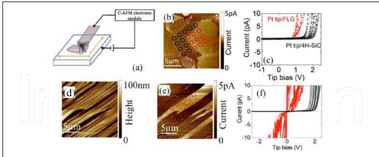
Fig. 18. Schematic representation of the Torsion Resonant-Conductive Atomic Force Microscopy (TR-CAF) setup (a). TR-CAF current map taken at tip bias of 1 V on deposited graphene on SiC (b). The brighter portions in the current map (region carrying a higher current) correspond to graphene coated regions. Local I - V curves measured on the indicated tip positions (c). TR-CAF morphology (d) and current (e) maps collected on EG on SiC. The investigated sample region is only partially covered with a single layer of epitaxial graphene. Local I - V characteristics collected in the same sample region (f). (Data from Ref. [48]).
