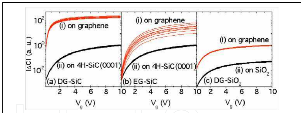
Fig. 14. Representative capacitance-voltage characteristics obtained on DG-SiC (a), EG-SiC (b) and DG-SiO 2 (c) on arrays of 5×5 tip positions with an inter-step distance of 1 \mu m×1 \mu m. (Data from Ref. [43]).
