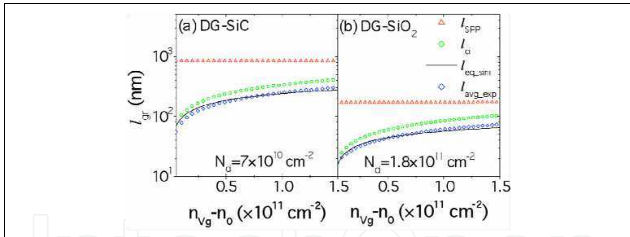
Fig. 16. Average of the l_{gr} vs n_{Vg} - n_0 curves measured on different tip positions on DG-SiC (a) and DG-SiO 2 (b). Data from Ref. [43].
