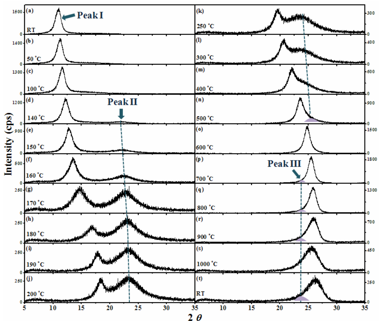
Fig. 4. Individual XRD plot for Fig. 3.
