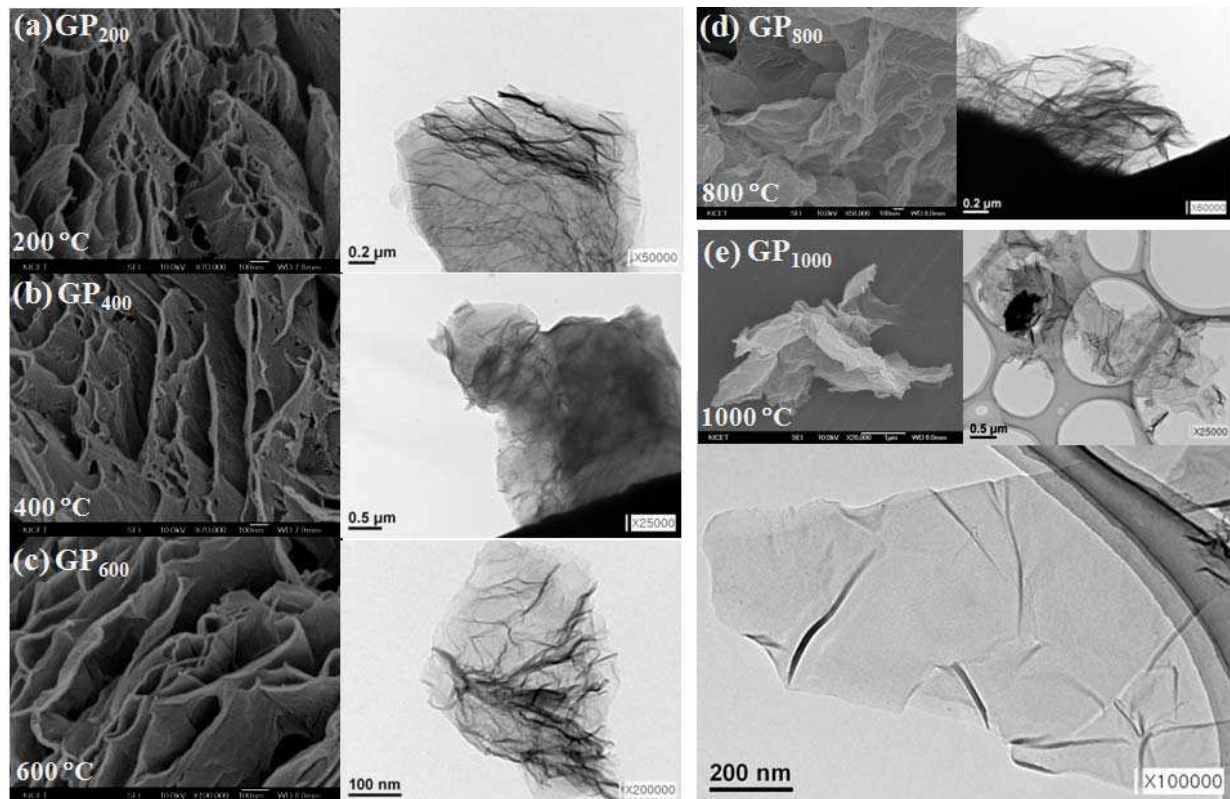
Fig. 12. FE-SEM (left) and FE-TEM images (right) for GP 200 (a), GP 400 (b), GP 600 (c), GP 800 (d), and GP 1000 (e).
