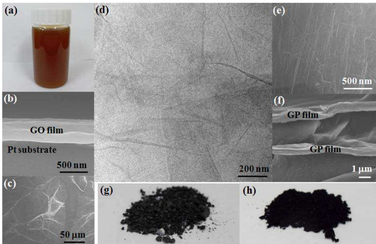
Fig. 2. A digital image of GO slurry (a), dried GO powder (g), and thermally reduced GP powder (h). FE-SEM images of GO films (b, c), thermally reduced GP films (e, f), and FE-TEM image of GO film (d).
