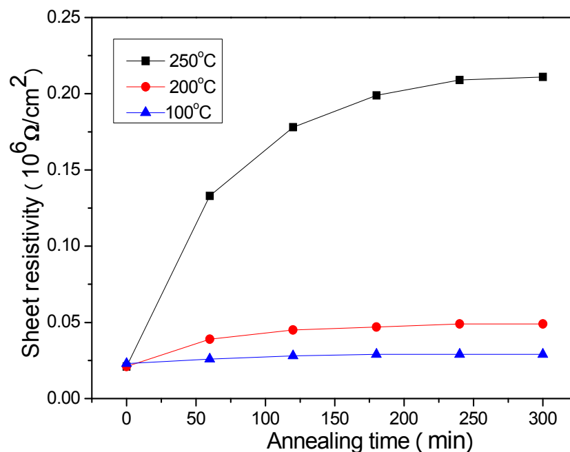
Fig. 10. Sheet resistivity against time of annealing
