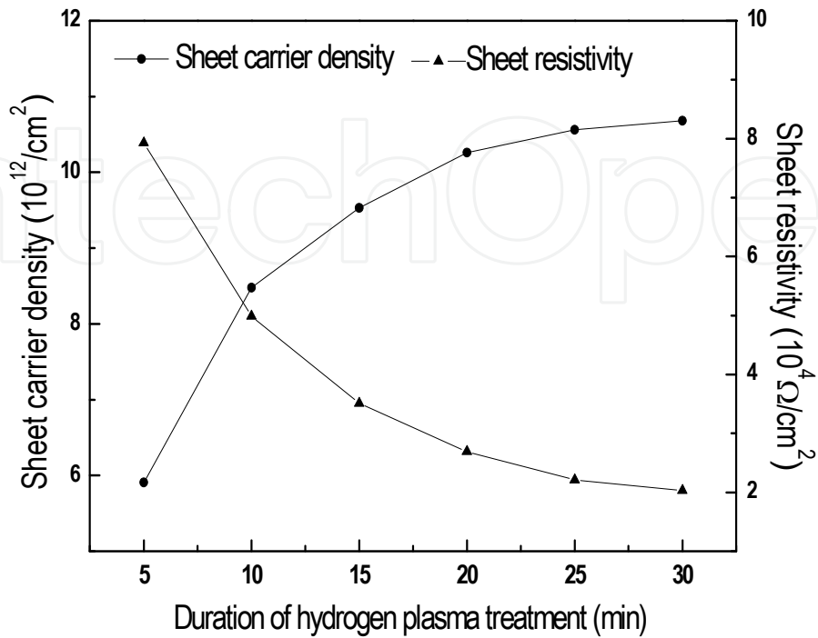
Fig. 6. Sheet carrier density and sheet resistivity of FSD against duration of hydrogen plasma treatment
