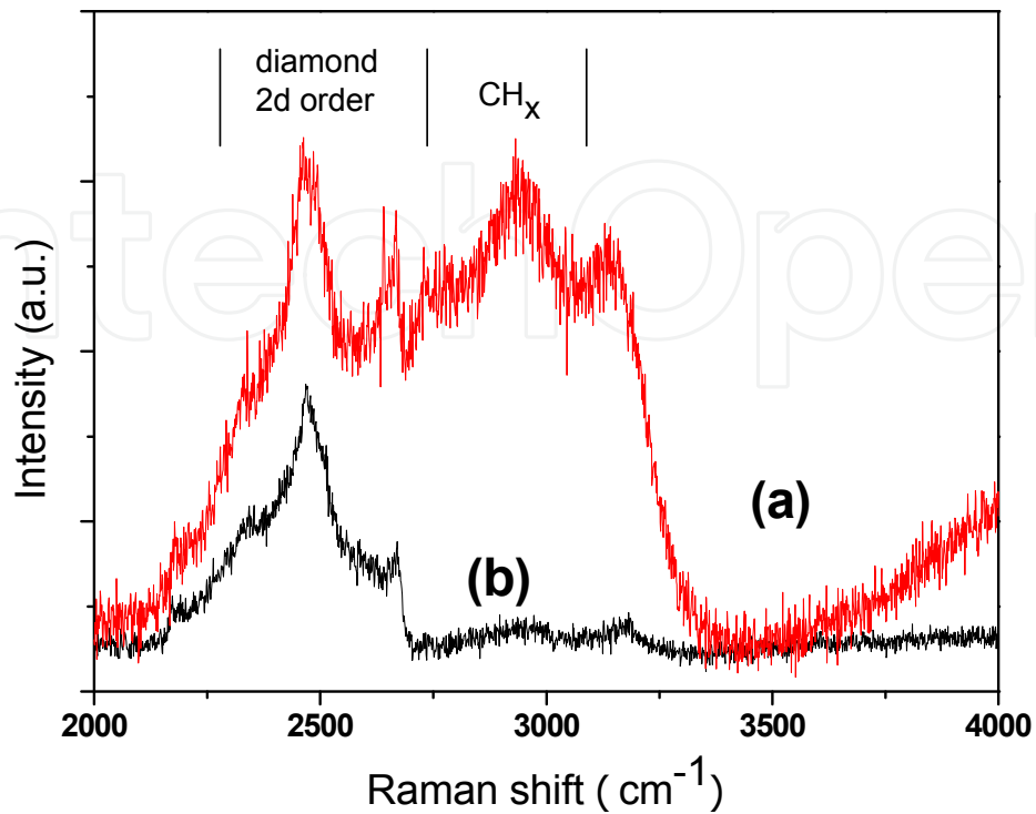
Fig. 11. Ultraviolet Raman scattering spectra for hydrogenated diamond nucleation surface sample (a) and annealed diamond surface sample (b)
