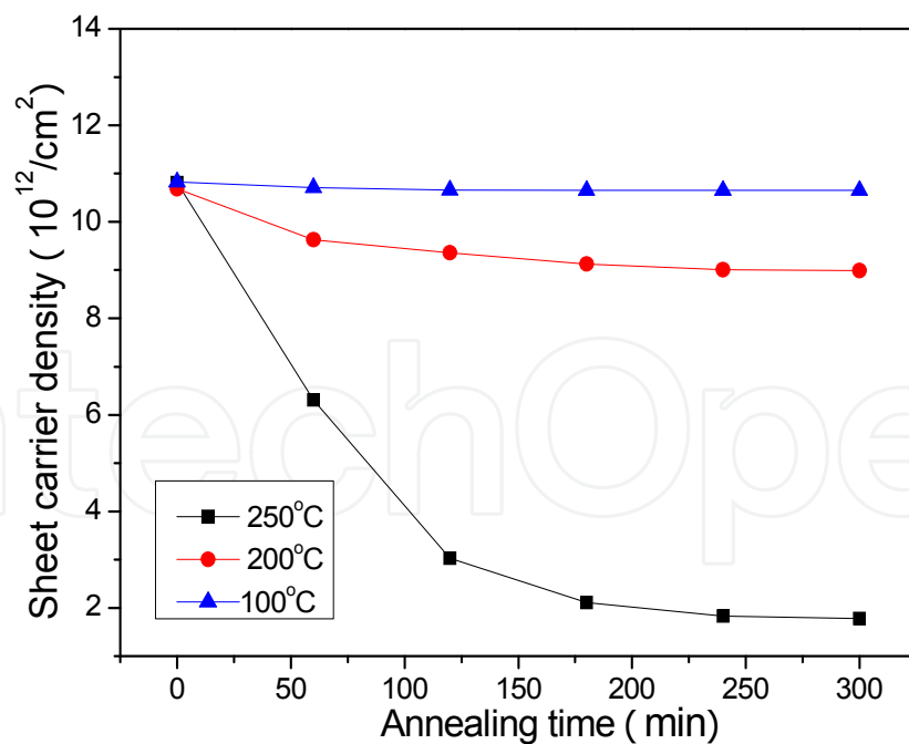
Fig. 9. Sheet carrier density against time of annealing
