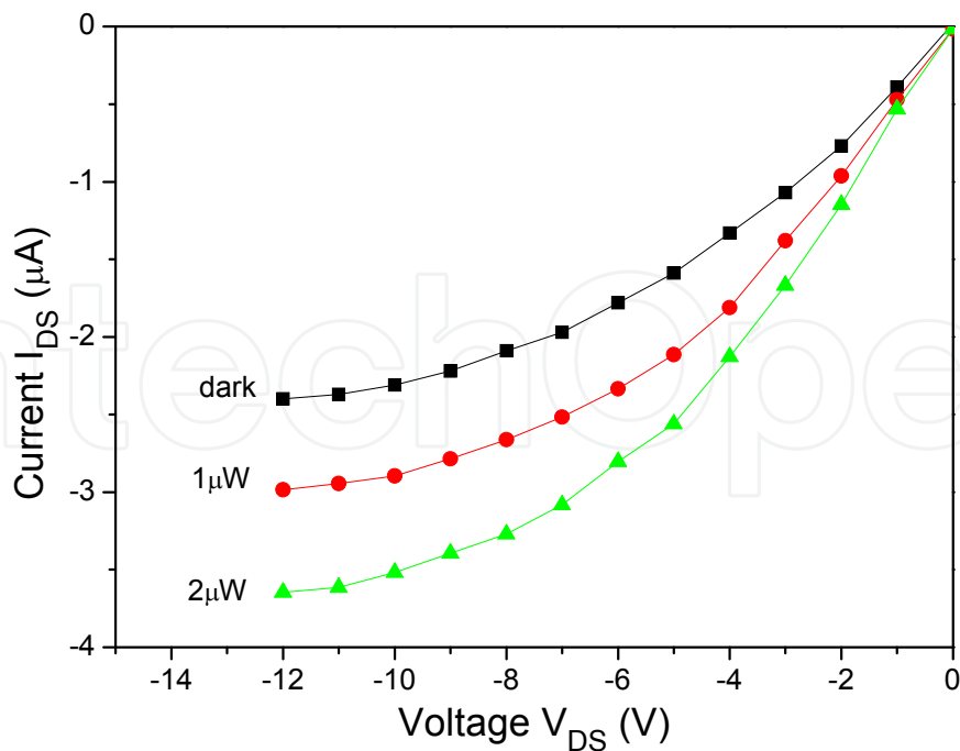
Fig. 18. Drain current against drain-source voltage for differing illumination power ( \lambda = 200 nm) with gate voltages of -0.1 V
