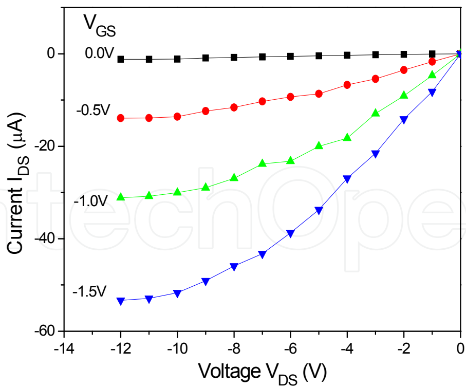
Fig. 17. Output characteristics of Hydrogen-terminated FSD film MESFET structures for negative bias. Drain-source voltage ( V_{DS} ) swept between 0 and -12 V; gate voltages ( V_{GS} ) swept between 0 and -1.5 V
