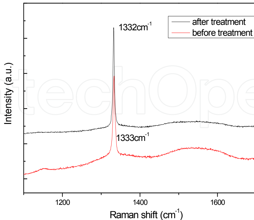
Fig. 5. Raman spectrum of nucleation side of freestanding diamond film
