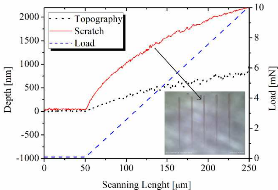
Fig. 8. Scratch test curve of SiO 2 layer of treated AryLite™ with optical image in the plot inset (magnification 20x). Topography and scratch scan refers to the third wear
