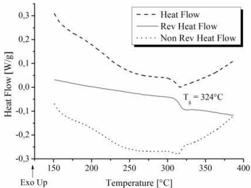
Fig. 3. Modulated Differential Scanning Calorimetry of AryLite™.
