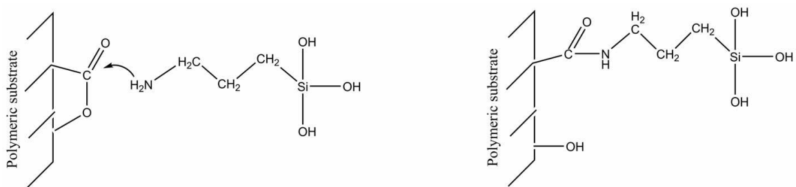
Fig. 1. Scheme of nucleophilic addition of NH 2 group to the polyester carbonic group
