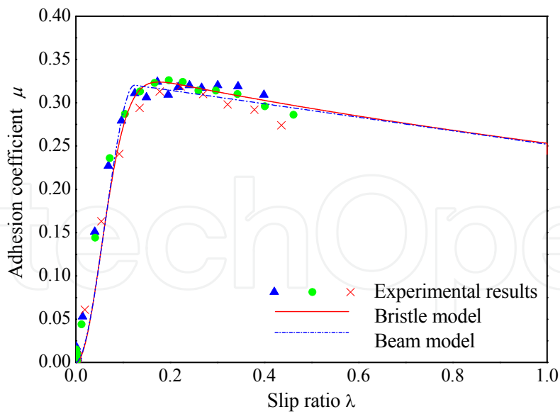
(c) Initial braking velocity v_0 = 60 km/h
