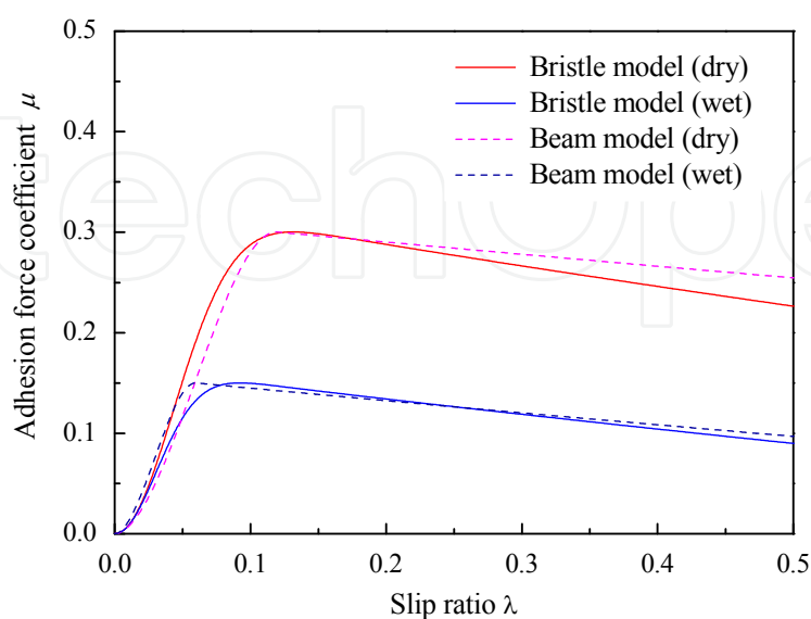
Fig. 17. Relationship between the adhesion force coefficient and the slip ratio according to the change in rail conditions from dry to wet based on the beam and bristle models.
