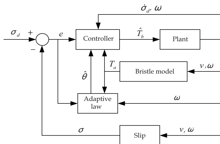
Fig. 16. Wheel-slip control system.
