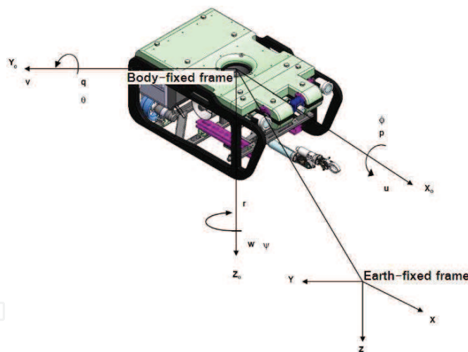
Fig. 2. Reference Earth-fixed frame and Body-fixed frame.
