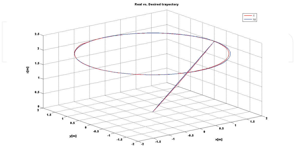
Fig. 7. Position tracking performance with SMC.
