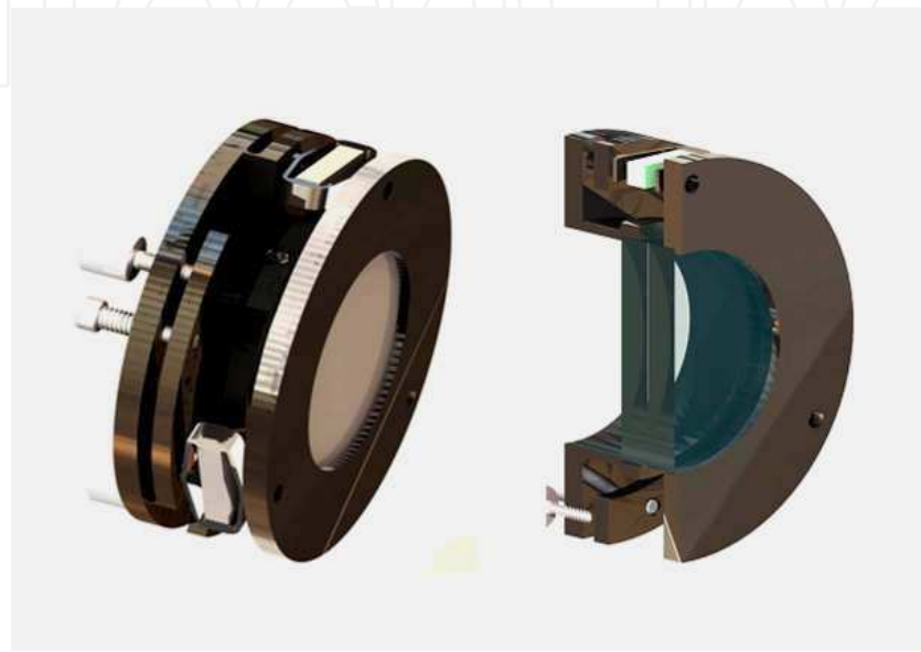
Fig. 15. Rendering of the F-P device and its section. The piezo actuator and the trimming screws are visible
