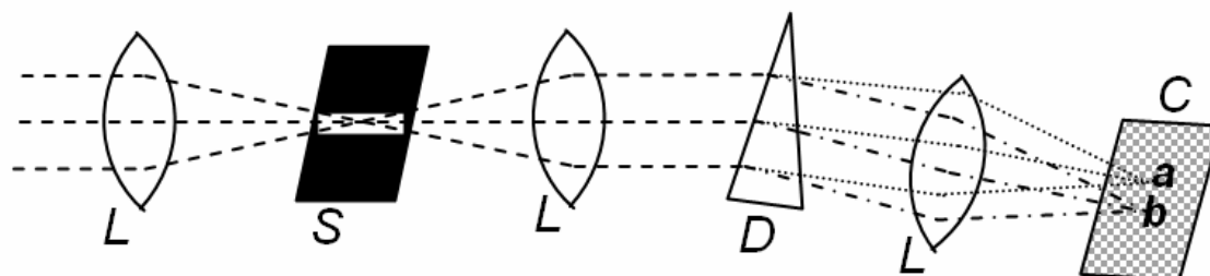
Fig. 1. Classical "pushbroom" hyperspectral imaging camera. L: collimating lenses, S: entrance slit selecting a row of the image in the focal plane; D: dispersive means (prism or grating) dispersing light in the direction orthogonal to the entrance slit; C: camera sensor where the combined image is focused. Points a and b , representing a pixel of the row selected at the entrance, are imaged at different vertical coordinates
