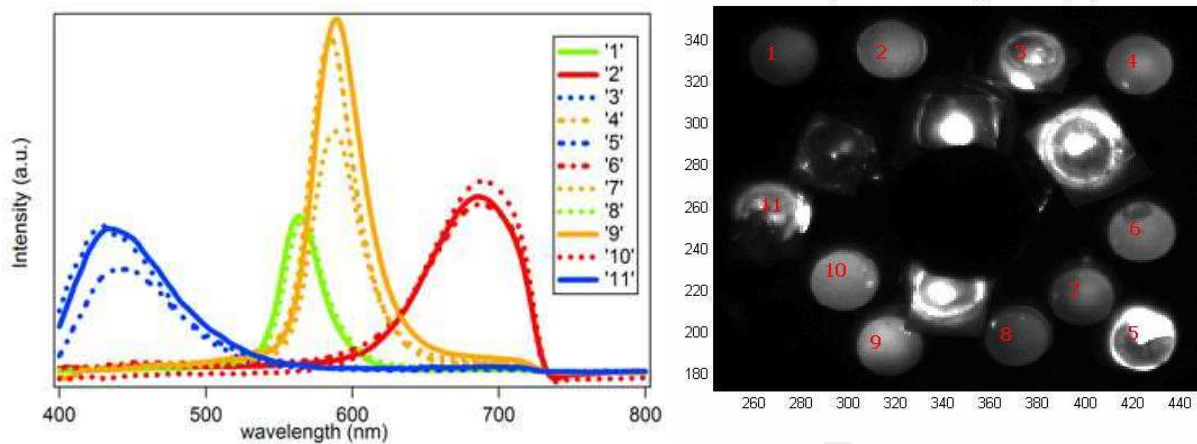
Fig. 21. The emission spectra on the left correspond to the pixel area ( 10 \times 10 ) indicated in the image on the right. The target is composed of LED of four different colors (blue, green, yellow and red)
