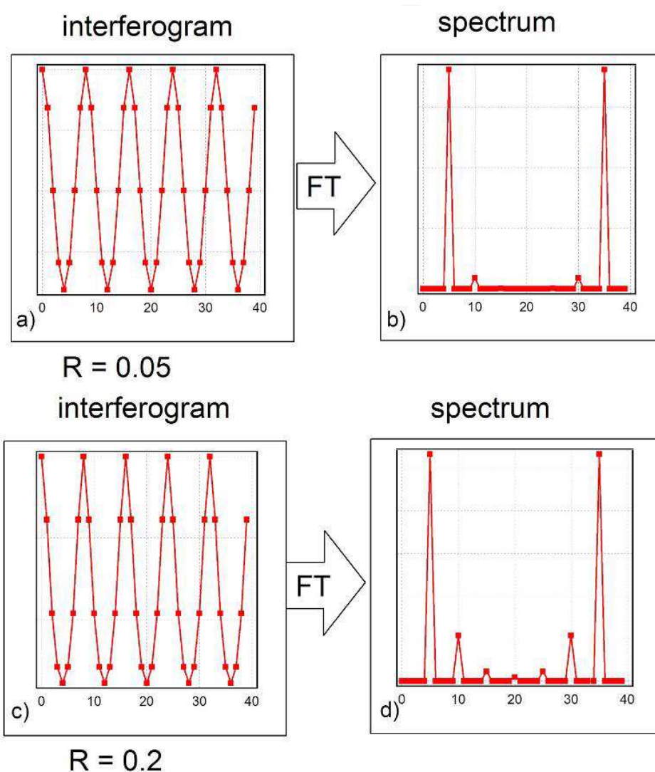
Fig. 6. Spectra obtained with DCT from F-P interferogram with different reflectivity. a) and b) interferogram and spectrum for reflectivity R = 0.05 . c) and d) interferogram and spectrum for reflectivity R = 0.2
