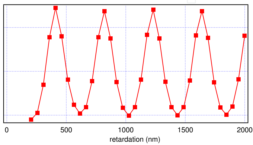
Fig. 8. The measured interferogram of a laser radiation at \lambda = 410 nm. The estimated penetration depth of the metallic layer is smaller than 50 nm
