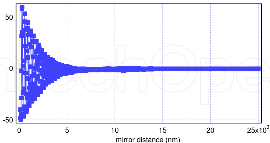
Fig. 9(a). The interferogram of a yellow LED with a maximum mirror distance \delta = 25 \mu\text{m}
