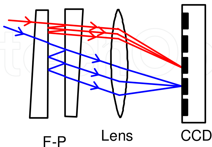
Fig. 4. Scheme of the F-P interferometer
