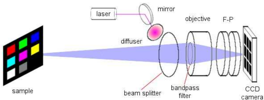
Fig. 16. Optical set-up formed by a beam splitter to couple the laser radiation to calibrate the retardation, the bandpass filter, the photographic objective and the CCD camera
