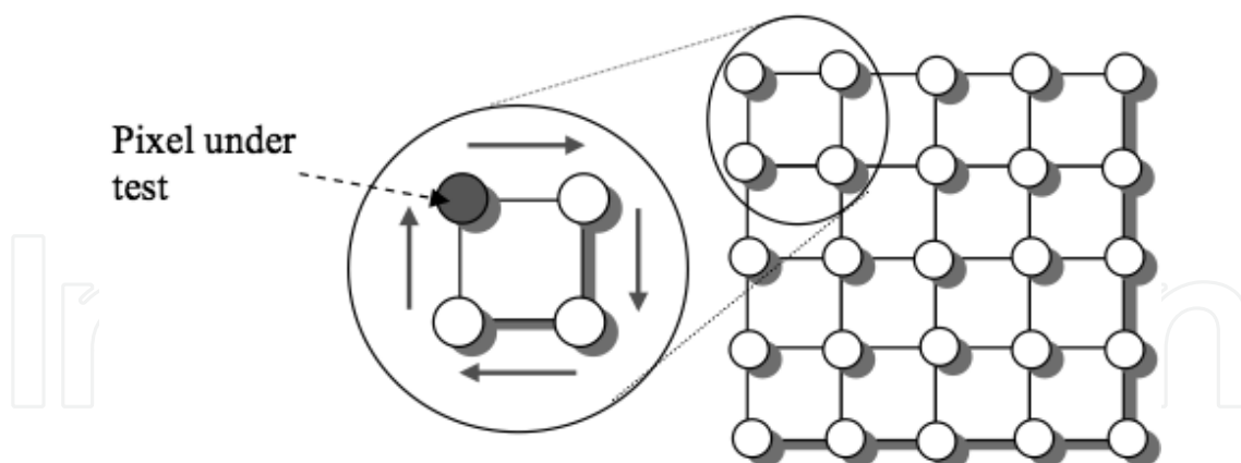
Fig. 4. Identifying residues in a 2 \times 2 closed path
