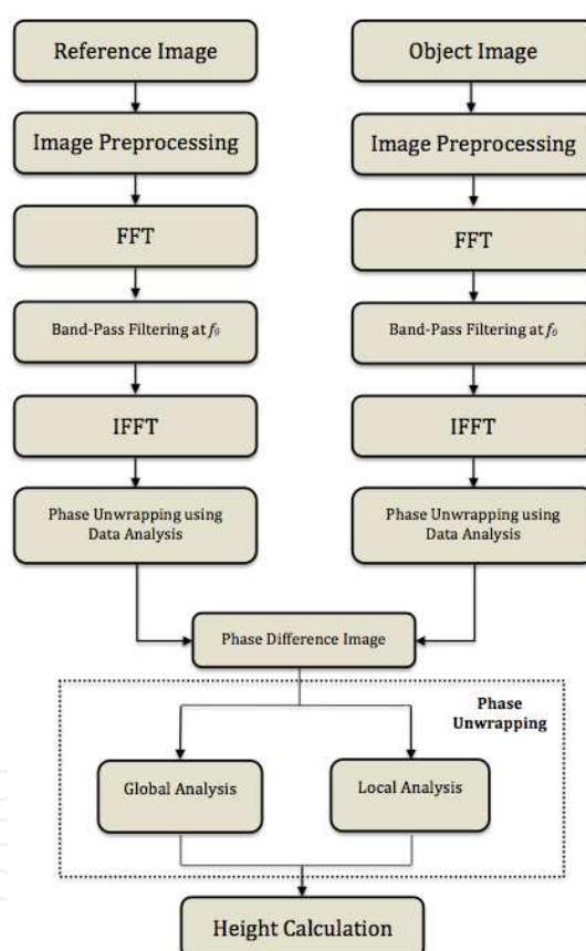
Fig. 3. Second Proposed Methodology
