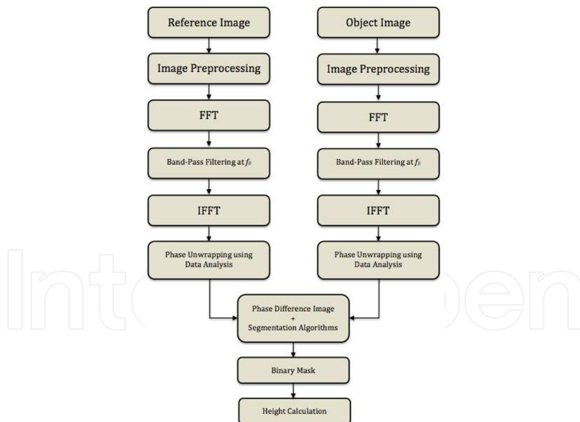
Fig. 2. Firstly Proposed Methodology
