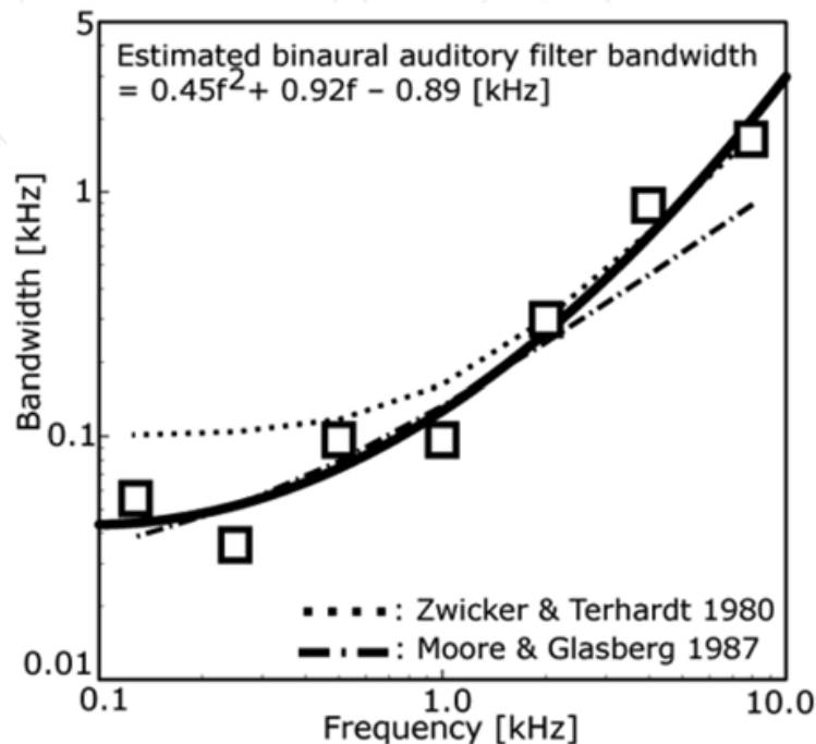
Fig. 3. The symbols ( \square ) indicate the estimates of the binaural auditory filter bandwidth from the N1m amplitudes at various center frequencies. The curve fitted to the data is specified by the equation in the figure. For comparison, the dotted line and dash-dot line show the the monaural CB function (Zwicker & Terhardt, 1980) and equivalent rectangular bandwidth of the auditory filter (Moore & Glasberg, 1987), respectively.
