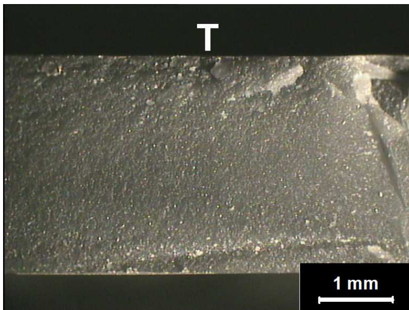
Fig. 12. Optical micrographs showing the planar fracture surface of the alumina monolithic laminate. The surface in tension in the flexure test is marked with T.
