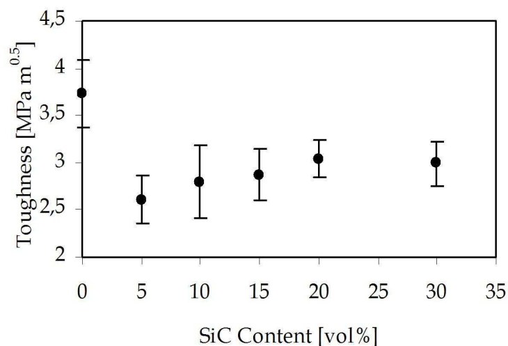
Fig. 9. Toughness of monolithic laminates.
