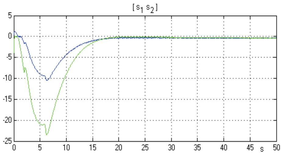
Fig. 3. Sliding functions
