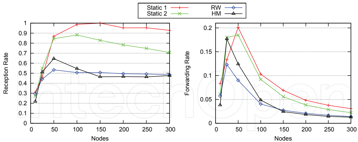
Fig. 5. Performance of MPR in a highway scenario with different mobility models and number of messages.
