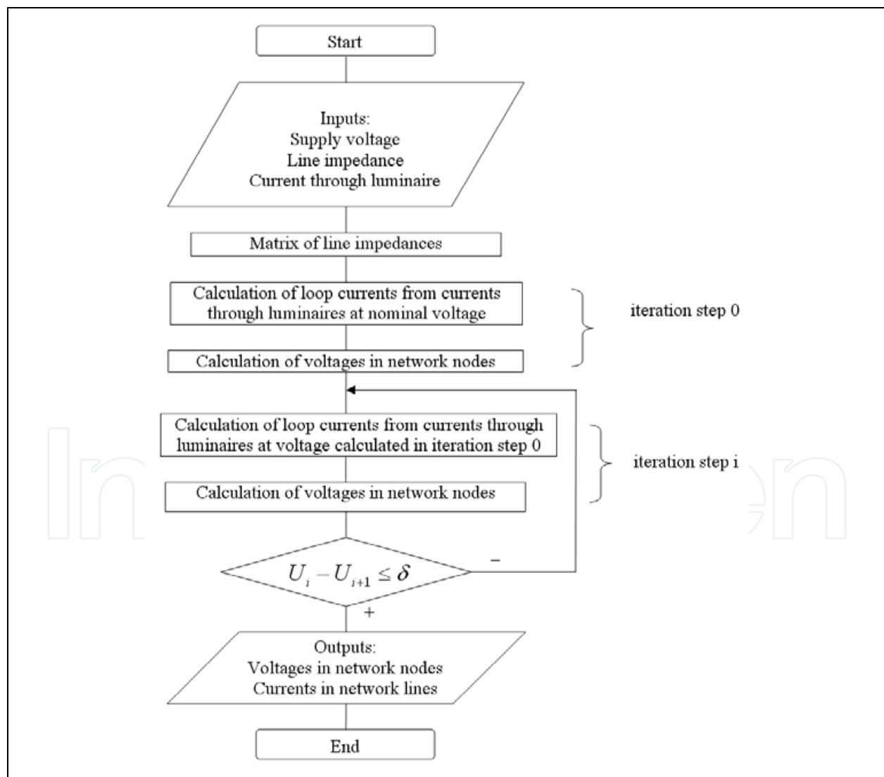
Fig. 21. Algorithm of calculation of steady-state public lighting network
