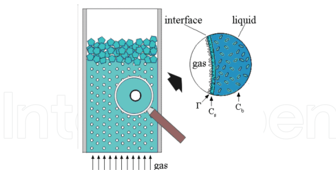
Fig. 4. Gas-liquid adsorption process in a bubble and foam column.
