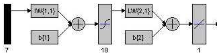
Fig. 7. Neural scheme implemented
