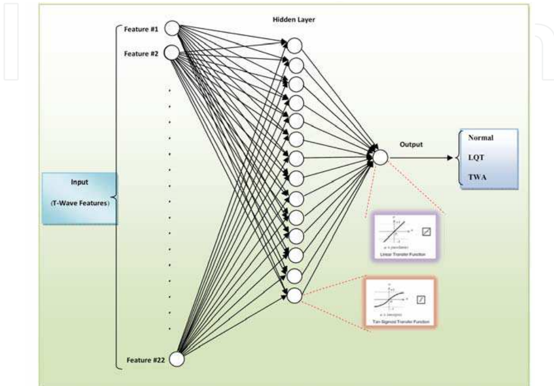
Fig. 10. Multi-layer perceptron (MLP) NN architecture.
