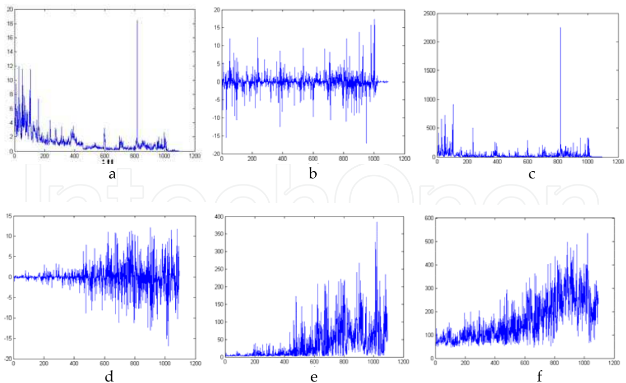
Fig. 13. BIS index versus : a) second central moment ( \mu_2 ), b) third central moment ( \mu_3 ), c) fourth central moment ( \mu_4 ), d) skewness (S), e) kurtosis (K), and f) the difference between maximum and minimum values of PDF ( \Delta )
