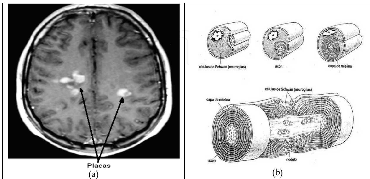
Fig. 3. Plaques (a) by the degeneration of myelin (b).
