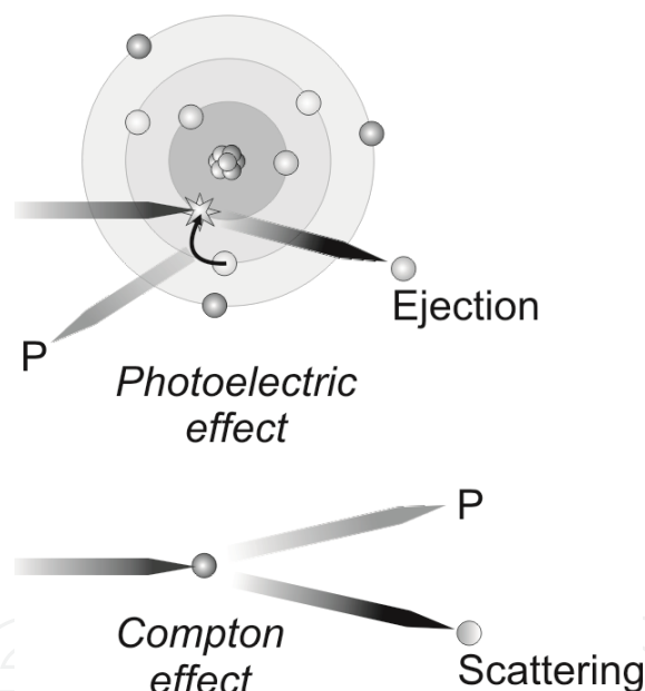
Fig. 1. The two main mechanisms of X-ray (blue line) attenuation are photoelectric effect and Compton effect. Photoelectric effect happens within electronic shells (layers) and consists in electron (colored sphere) ejection with concomitant emission of photon and reorganisation of electrons between shells. Compton effect happens with electrons which are scattered with concomitant emission of photon.
