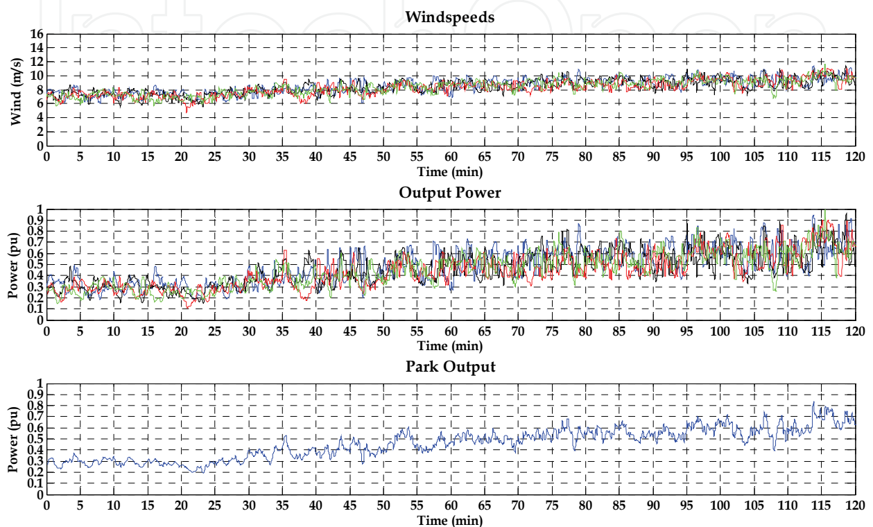
Fig. 25. Wind profiles; Turbines output; Park total output
