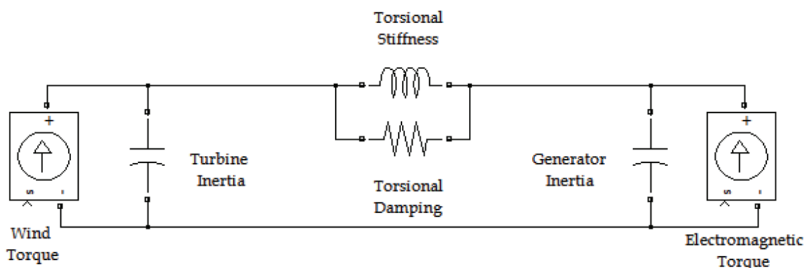
Fig. 9. Electrical equivalent of the two masses shaft.
