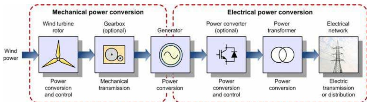
Fig. 2. General description of a wind turbine system
