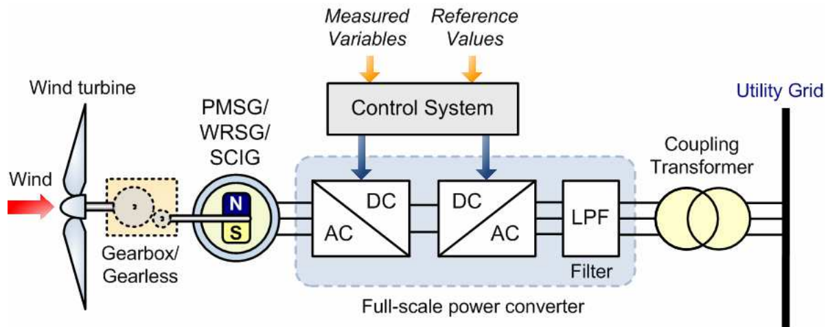
Fig. 7. Type D wind turbine concept: Direct-in-line variable speed wind turbine connected to the electric grid through a full-scale power converter
