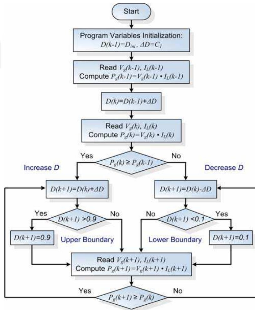
Fig. 14. Flowchart for the P&O MPPT algorithm
