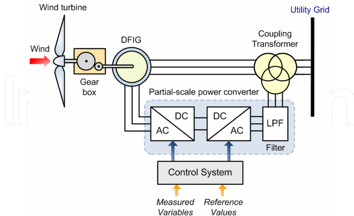
Fig. 6. Type C wind turbine concept: Variable speed wind turbine directly connected to the electric grid via a doubly-fed induction generator controlled with a partial-scale power converter
