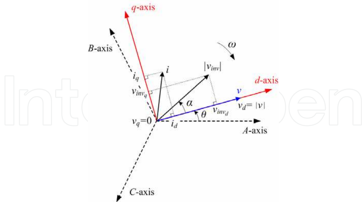
Fig. 12. Voltage source inverter vectors in the synchronous rotating d - q reference frame Thus,
