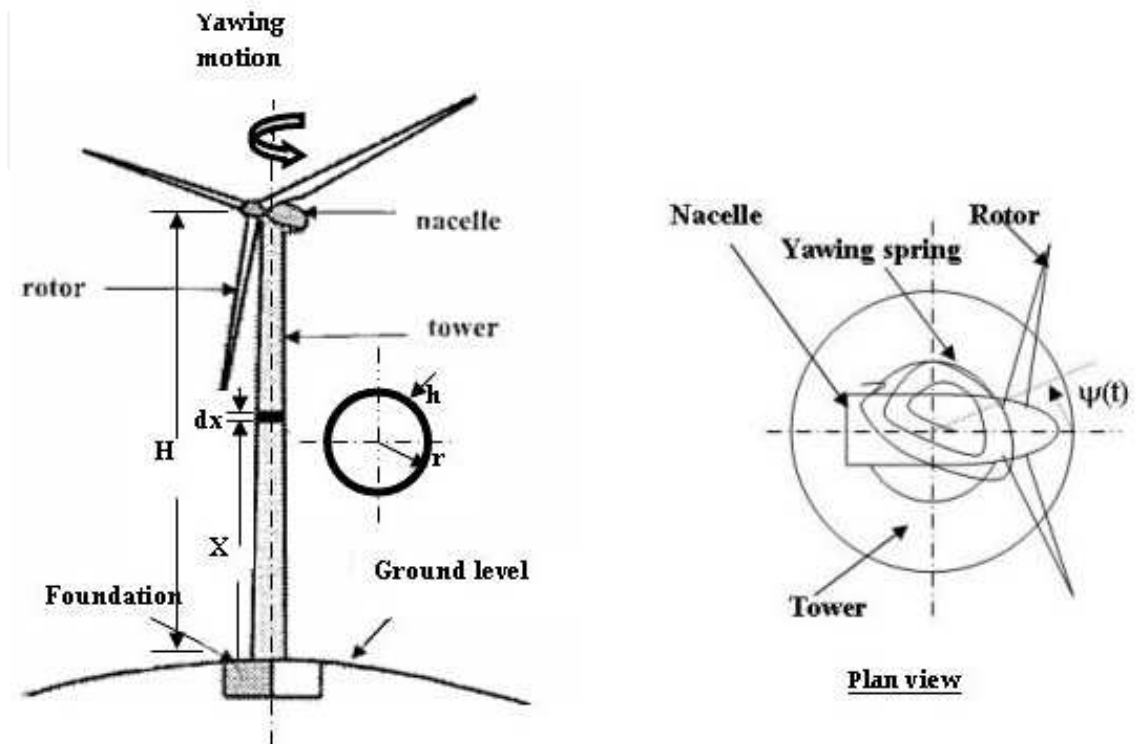
Fig. 5. Horizontal-axis wind turbine in free yawing motion
