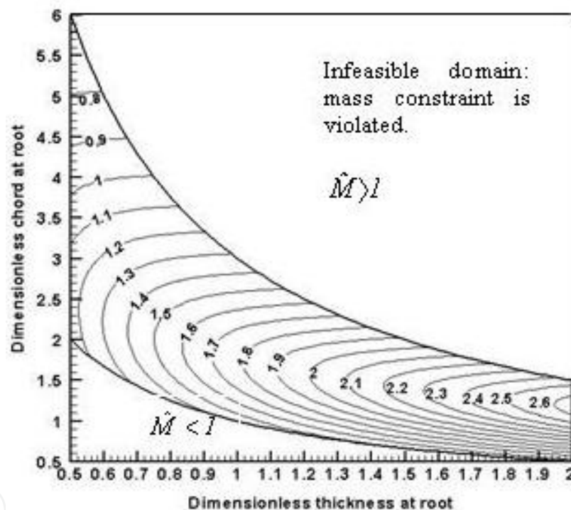
Fig. 9. Augmented pitching frequency-mass contours ( \hat{\omega}_1 ) for a blade with flexible root: \hat{K}_s = 10 ( \hat{M} = 1 )
