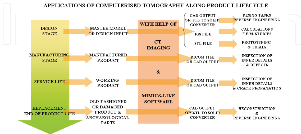
Fig. 1. Schematic review of applications of computerized tomography for product lifecycle.
