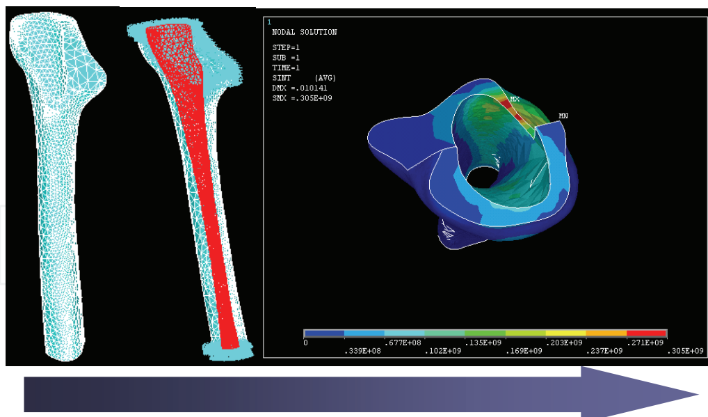
Fig. 8. Example of mechanical FEM study based on the information from CT images.
