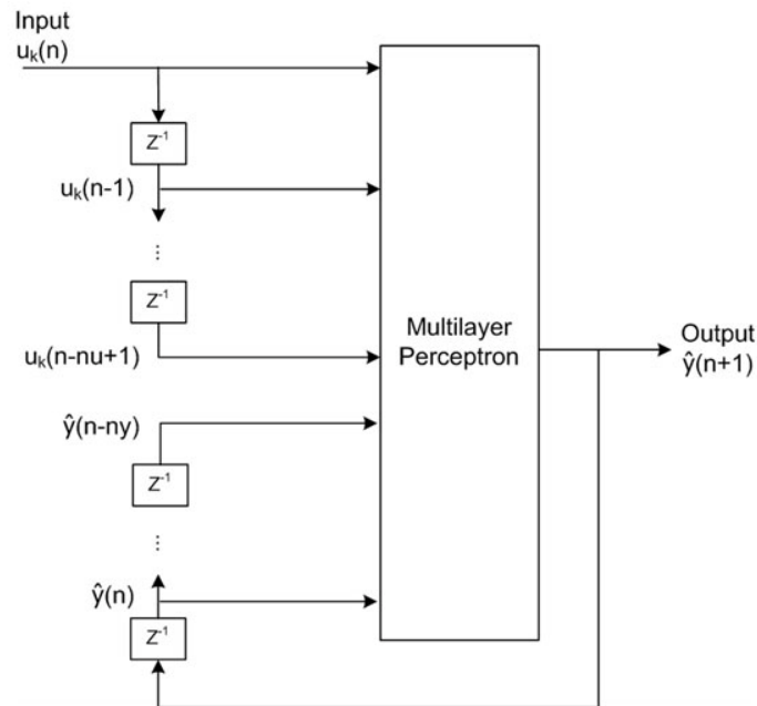
Fig. 1. Canonical representation of a NLARX model structure
