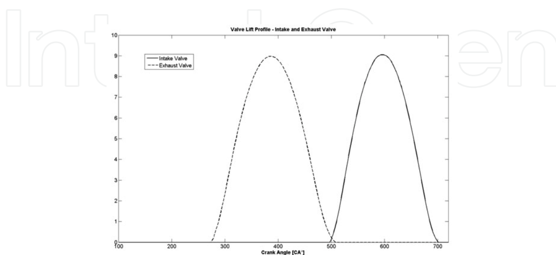
Fig. 17. Valve-Lift profile for inlet and exhaust valve
