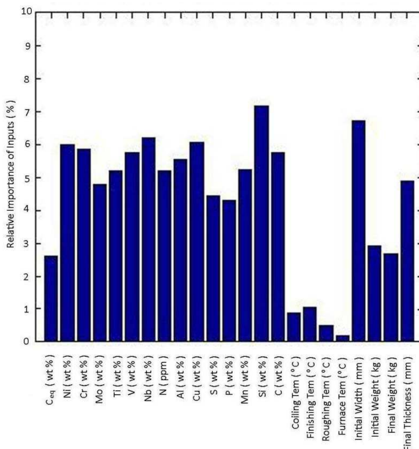
Fig. 6. Relative importance of inputs.
