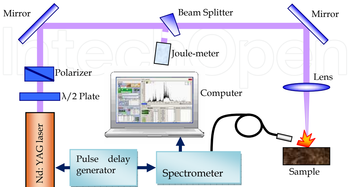
Fig. 1. Experimental configuration of a LIBS system.
