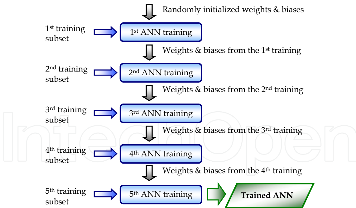
Fig. 8. Sequential training diagram.
