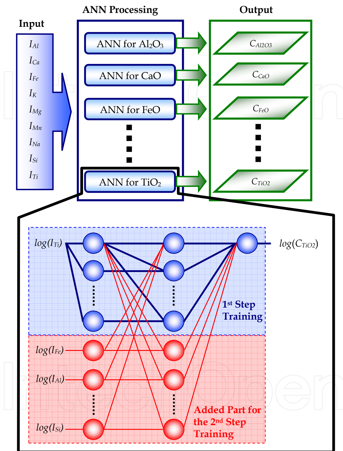
Fig. 13. Architecture of the expanded ANN for the constructive training. The blue dashed box indicates the structure of the ANN corresponding to the 1 st step training. The red dashed box shows the neurons and connections added to the initial network (blue) during the 2 nd training (constructive). In the 2 nd training, the weights and biases of the blue neurons are initialised with the values obtained from the first training, while the weights and biases of the red neurons are initialised with small values much lower than those of blue neurons.
