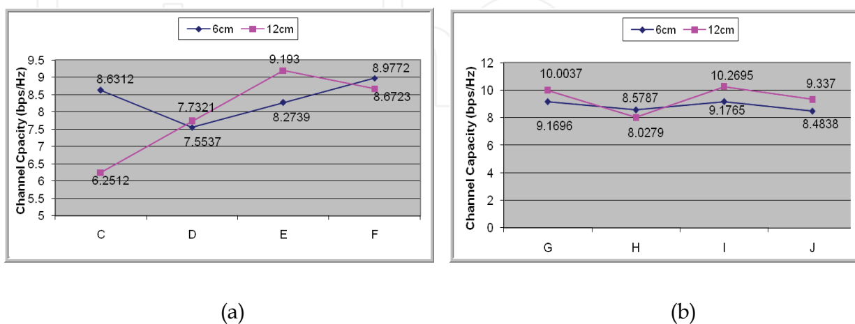
Fig. 6. (a) Average Channel Capacity for Polarization Diversity at Transmitter Fig. 6 (b). Average Channel Capacity for Polarization Diversity at Receiver
