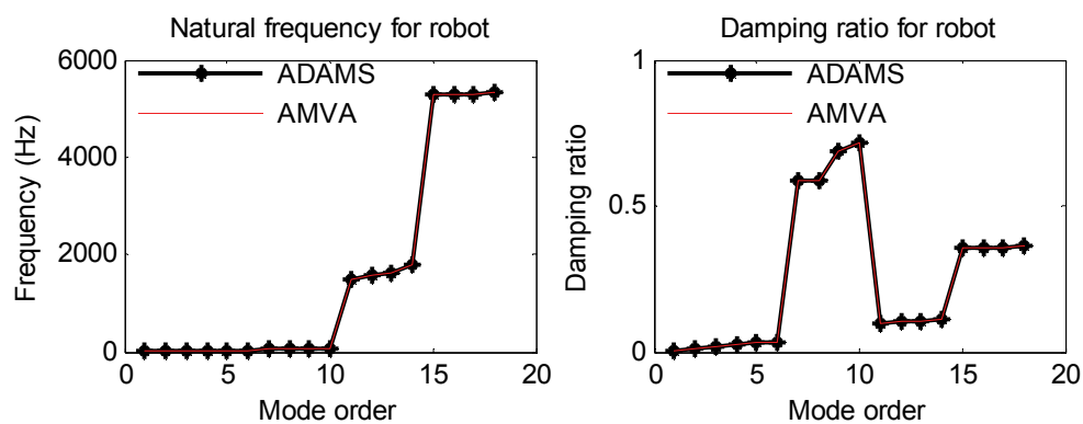
Fig. 10. Comparison of NMA results for quadruped robot
