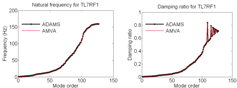
Fig. 7. Comparison of NMA results for model TL7RF1
