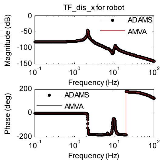
Fig. 11. Comparison of TFA results for quadruped robot
