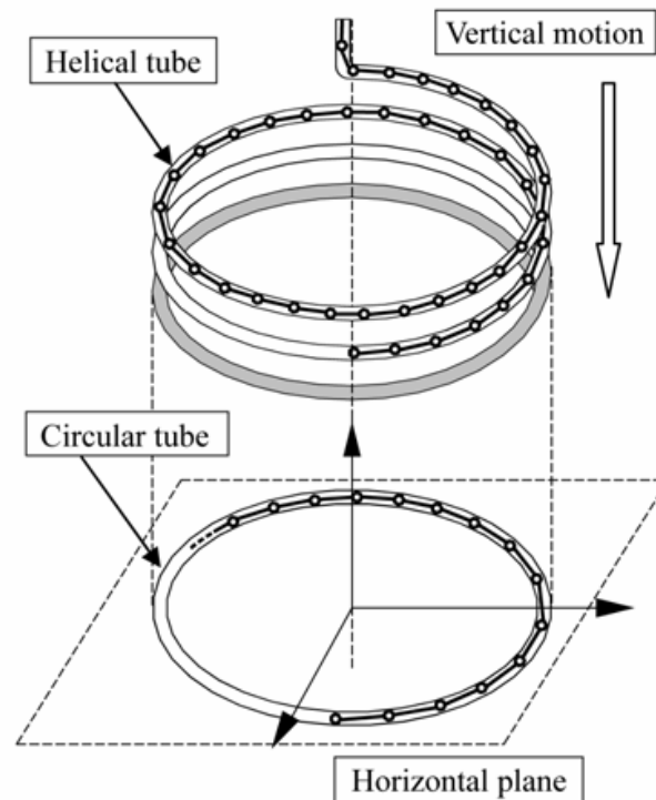
Fig. 6. Actual and analytical heating tube.
