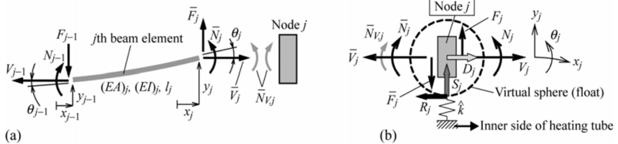
Fig. 9. State variables and external forces at (a) both ends of the j th beam element and (b) node j .
