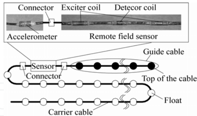
Fig. 2. ECT probe and accelerometer.
