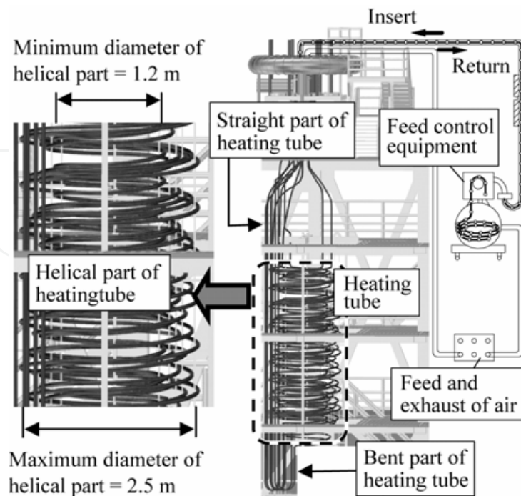
Fig. 1. Mock-up test facility.
